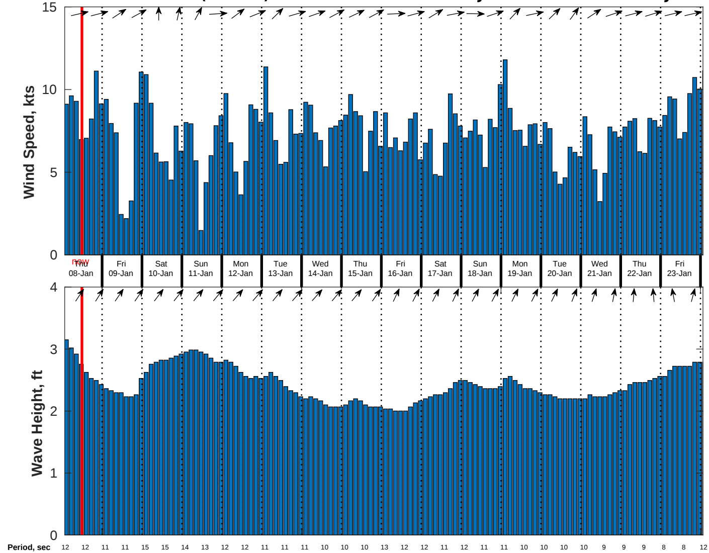
Wind & Wave Forecast for CSA (ONHYM) PPL EBS - Liberia from 07-Jan-2026 01:00:00 to 23-Jan-2026 01:00:00
