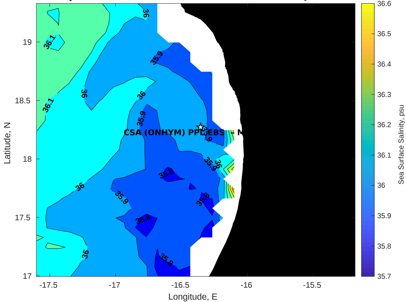
Surface Salinity for CSA (ONHYM) PPL EBS - Mauritania at 06-Jan-2026 00:00:00
