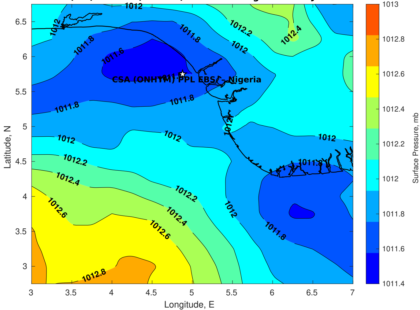
Surface Pressure (mb) for CSA (ONHYM) PPL EBS - Nigeria at 08-Jan-2026 00:00:00
