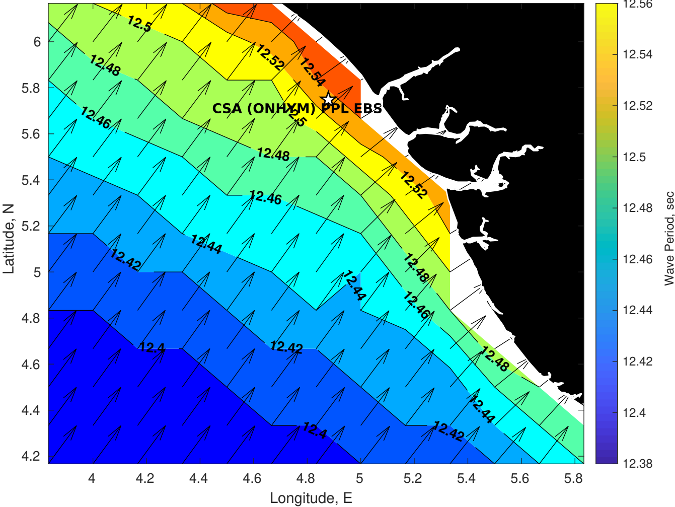
GFS Wave Period (sec) for CSA (ONHYM) PPL EBS - Nigeria at 07-Jan-2026 09:00:00
