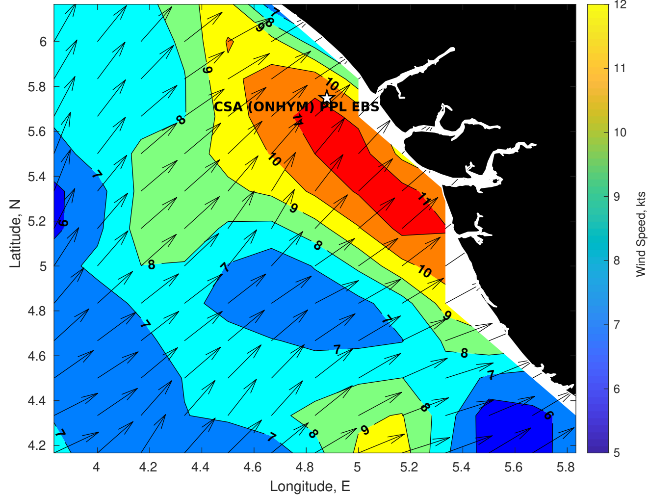
GFS Winds (kts) for CSA (ONHYM) PPL EBS - Nigeria at 07-Jan-2026 09:00:00
