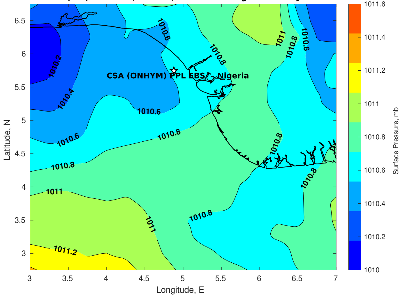
Surface Pressure (mb) for CSA (ONHYM) PPL EBS - Nigeria at 07-Jan-2026 00:00:00
