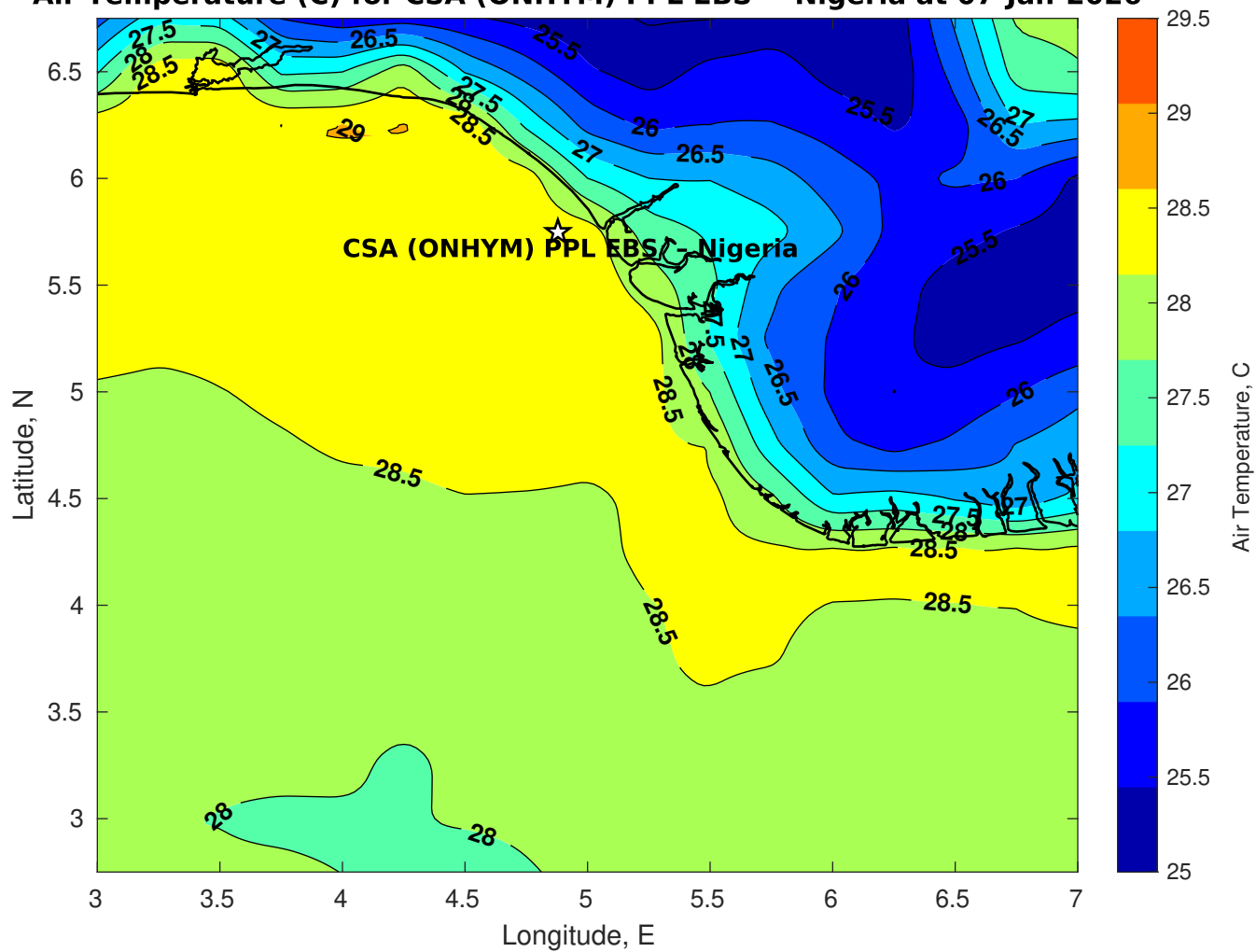
Air Temperature (C) for CSA (ONHYM) PPL EBS - Nigeria at 07-Jan-2026
