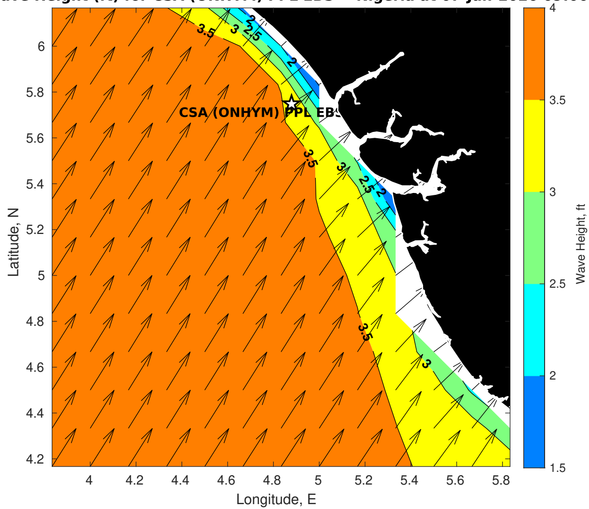
GFS Wave Height (ft) for CSA (ONHYM) PPL EBS - Nigeria at 07-Jan-2026 09:00:00
