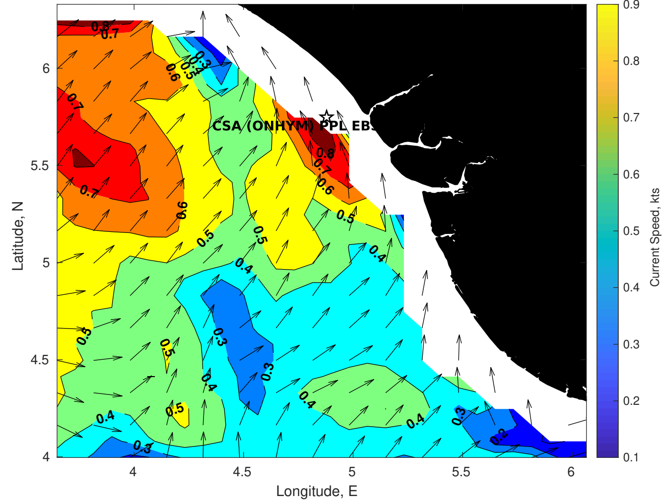
Surface Currents for CSA (ONHYM) PPL EBS - Nigeria at 06-Jan-2026 00:00:00
