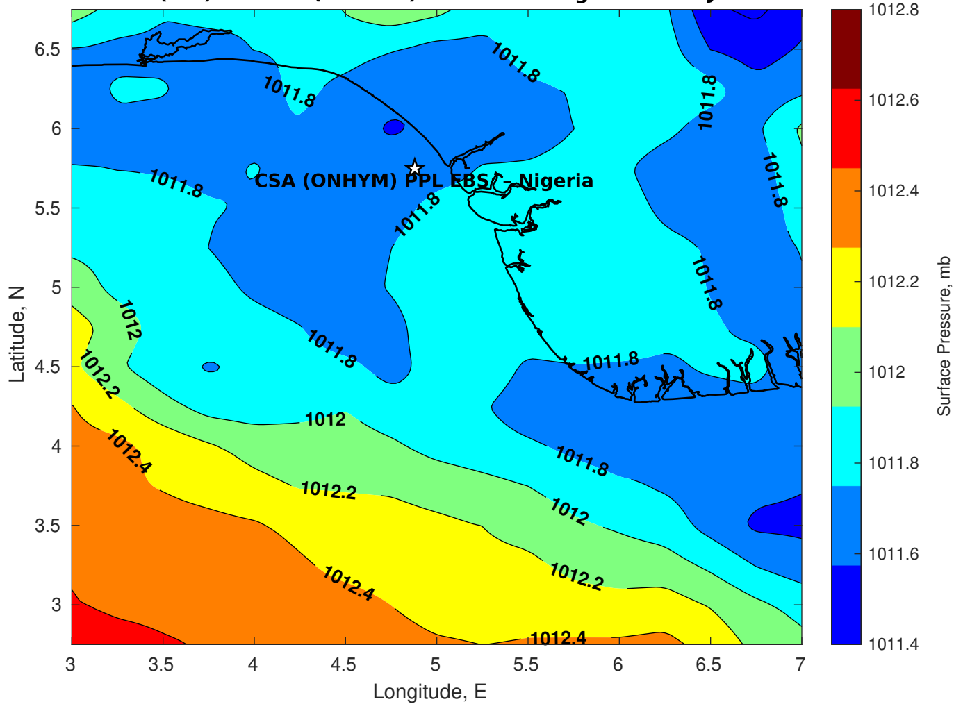
Surface Pressure (mb) for CSA (ONHYM) PPL EBS - Nigeria at 09-Jan-2026 00:00:00
