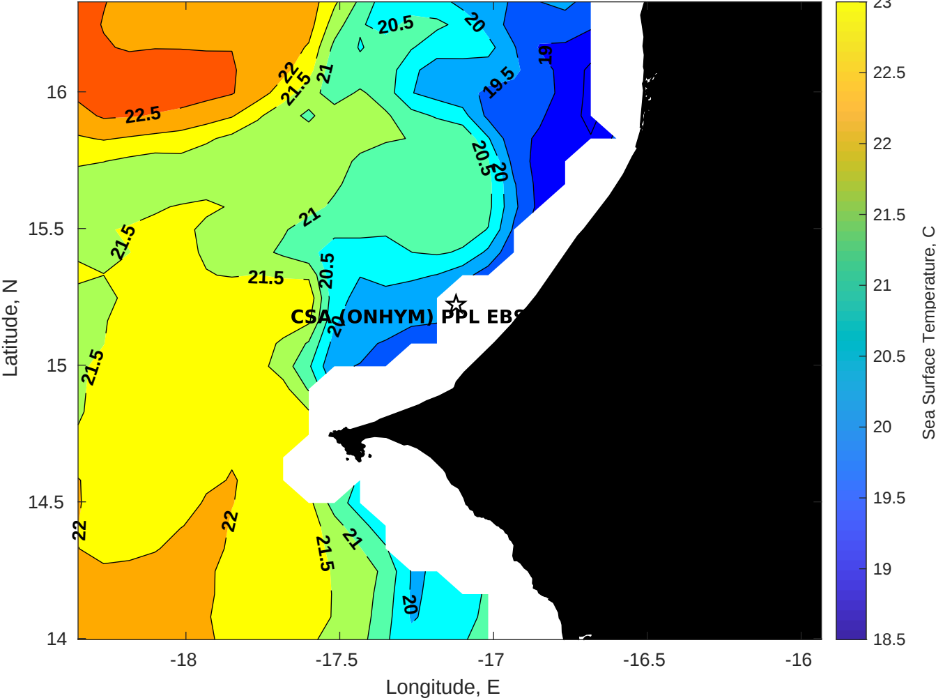
SST for CSA (ONHYM) PPL EBS - Senegal at 06-Jan-2026 00:00:00
