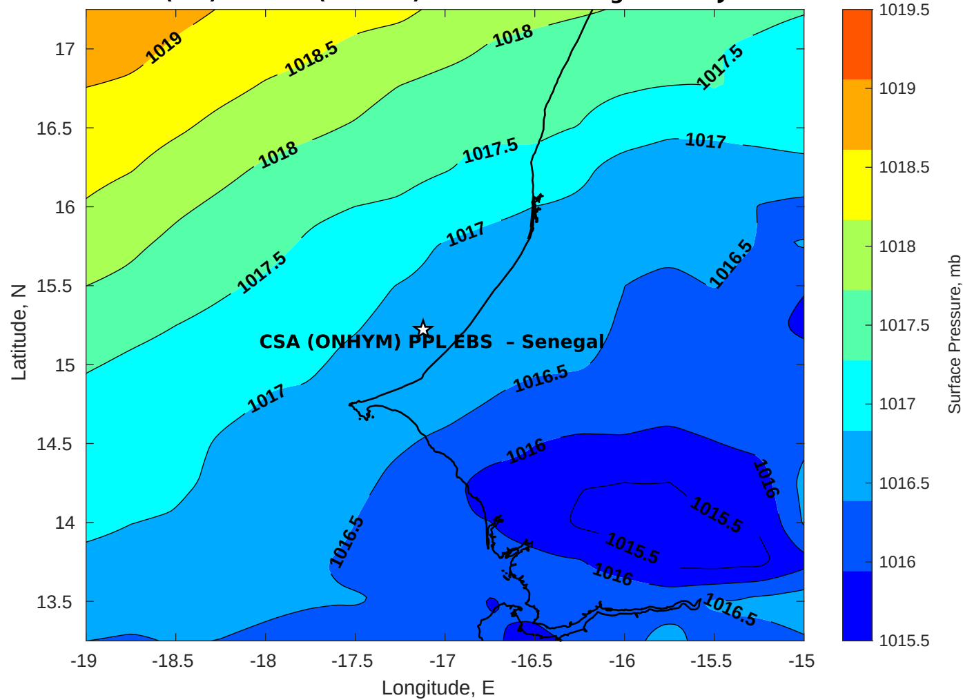
Surface Pressure (mb) for CSA (ONHYM) PPL EBS - Senegal at 08-Jan-2026 00:00:00
