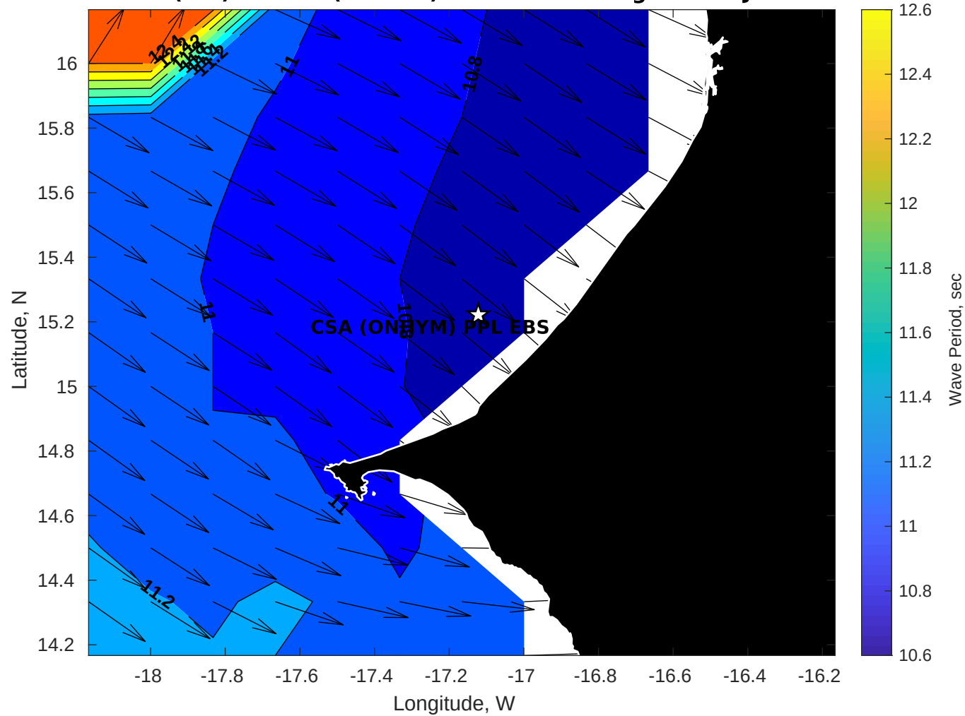
GFS Wave Period (sec) for CSA (ONHYM) PPL EBS - Senegal at 07-Jan-2026 09:00:00
