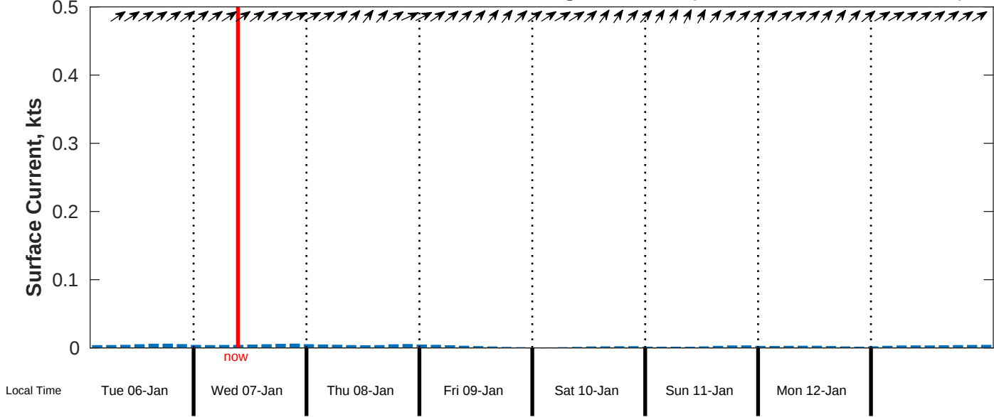
Surface Current Forecast for CSA (ONHYM) PPL EBS - Senegal from 06-Jan-2026 00:00:00 to 14-Jan-2026 00:00:00
