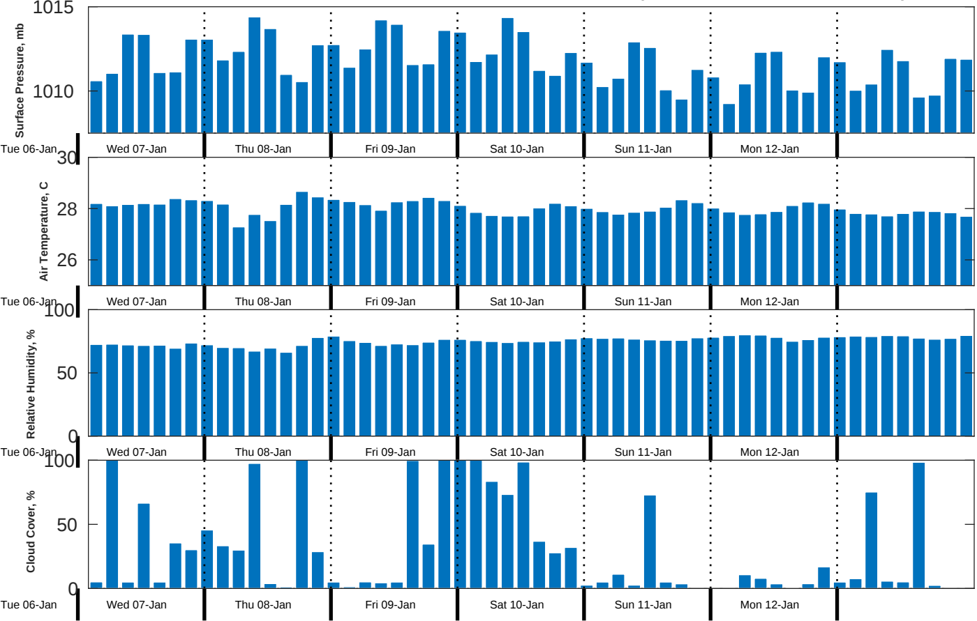
Met Forecast for CSA (ONHYM) PPL EBS - Sierra Leone from 07-Jan-2026 00:00:00 to 14-Jan-2026 00:00:00
