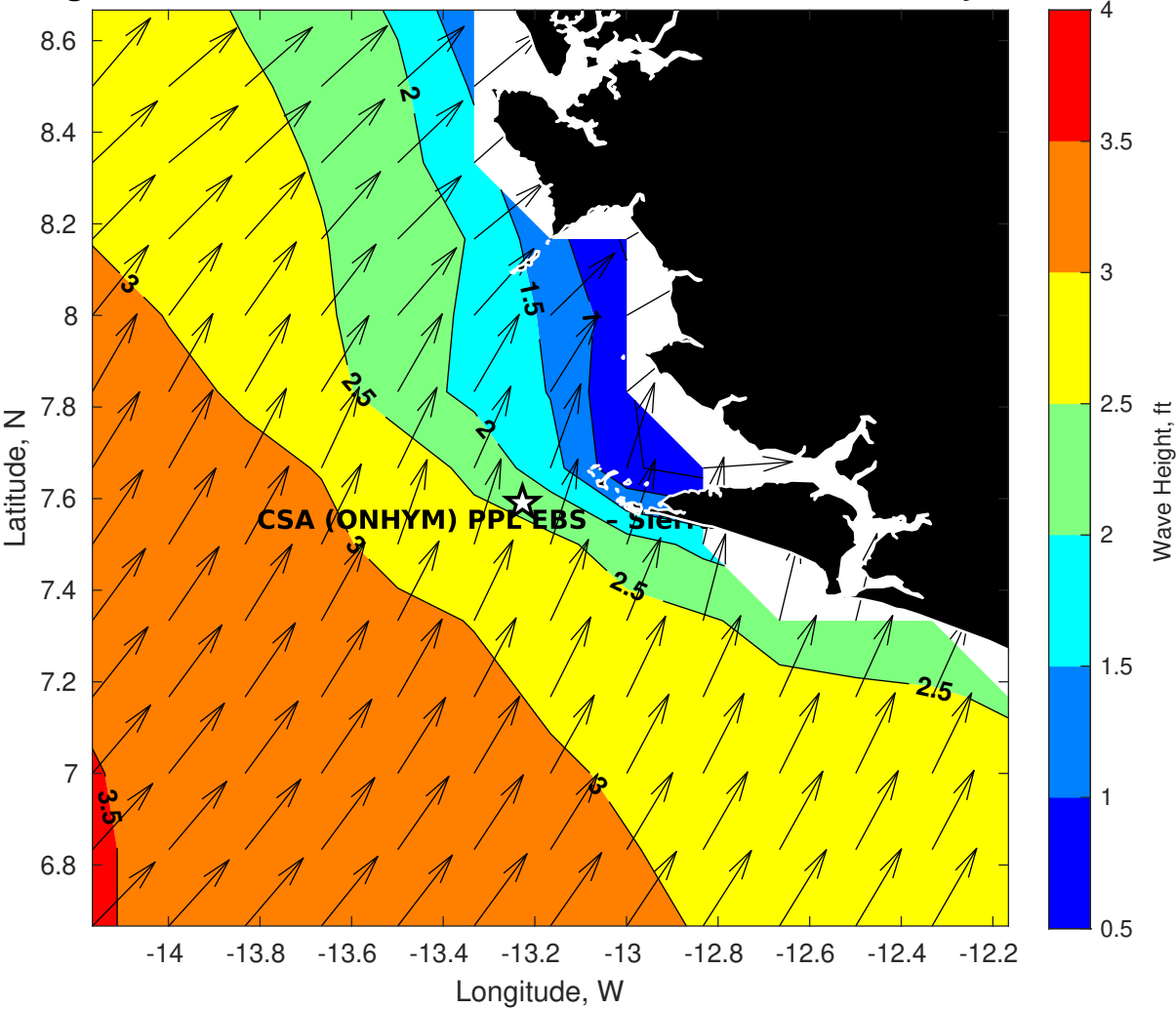
GFS Wave Height (ft) for CSA (ONHYM) PPL EBS - Sierra Leone at 07-Jan-2026 09:00:00
