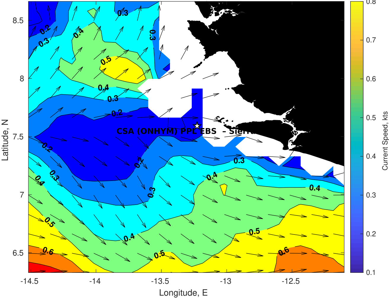
Surface Currents for CSA (ONHYM) PPL EBS - Sierra Leone at 06-Jan-2026 00:00:00
