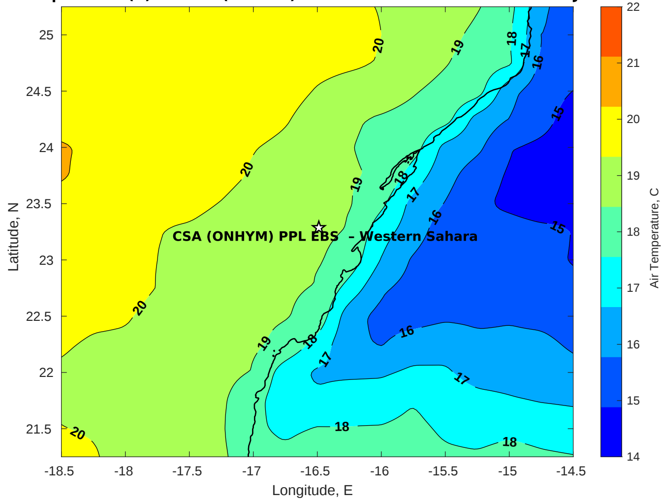
Air Temperature (C) for CSA (ONHYM) PPL EBS - Western Sahara at 07-Jan-2026
