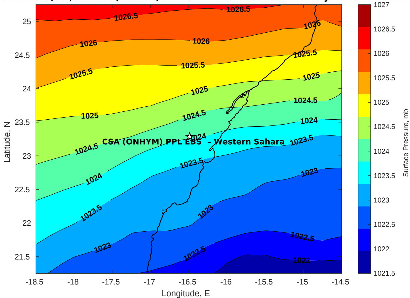
Surface Pressure (mb) for CSA (ONHYM) PPL EBS - Western Sahara at 08-Jan-2026 00:00:00
