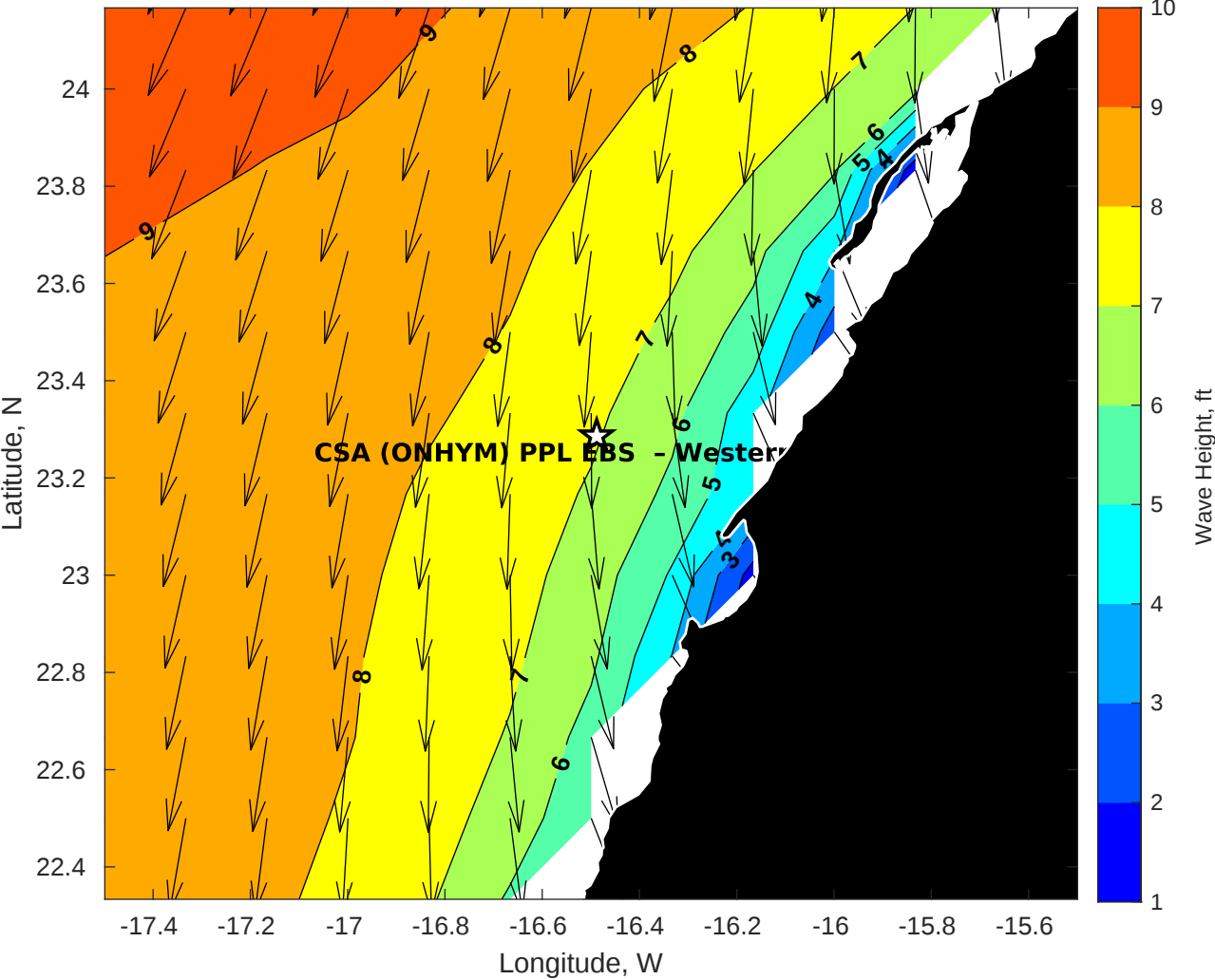
GFS Wave Height (ft) for CSA (ONHYM) PPL EBS - Western Sahara at 07-Jan-2026 09:00:00
