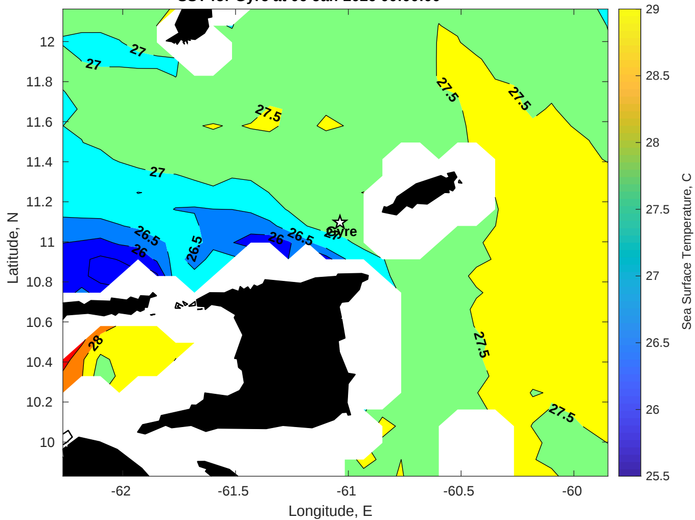
SST for Gyre at 06-Jan-2026 00:00:00
