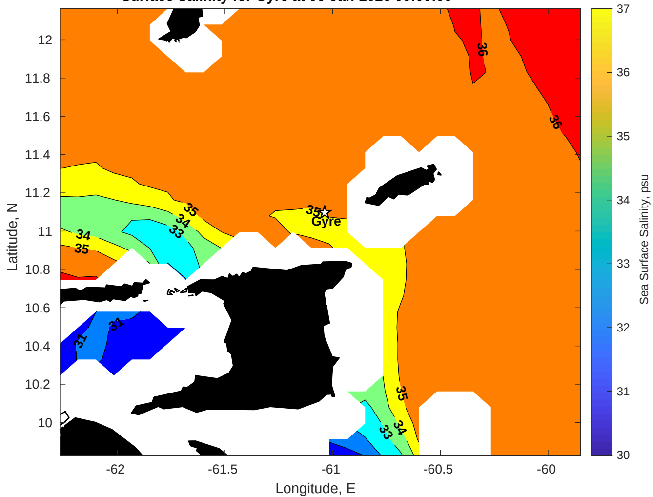
Surface Salinity for Gyre at 06-Jan-2026 00:00:00
