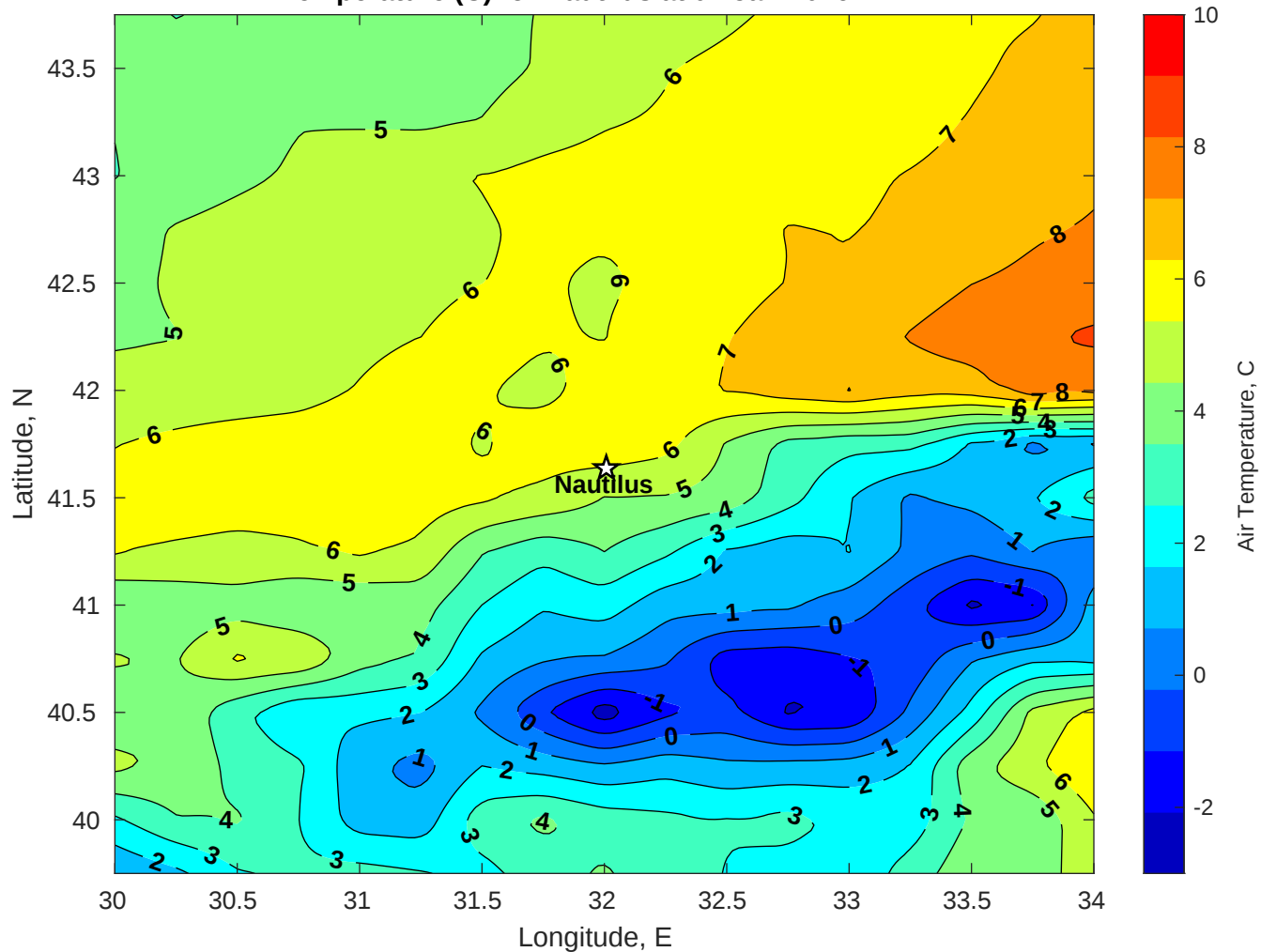
Air Temperature (C) for Nautilus at 07-Jan-2026
