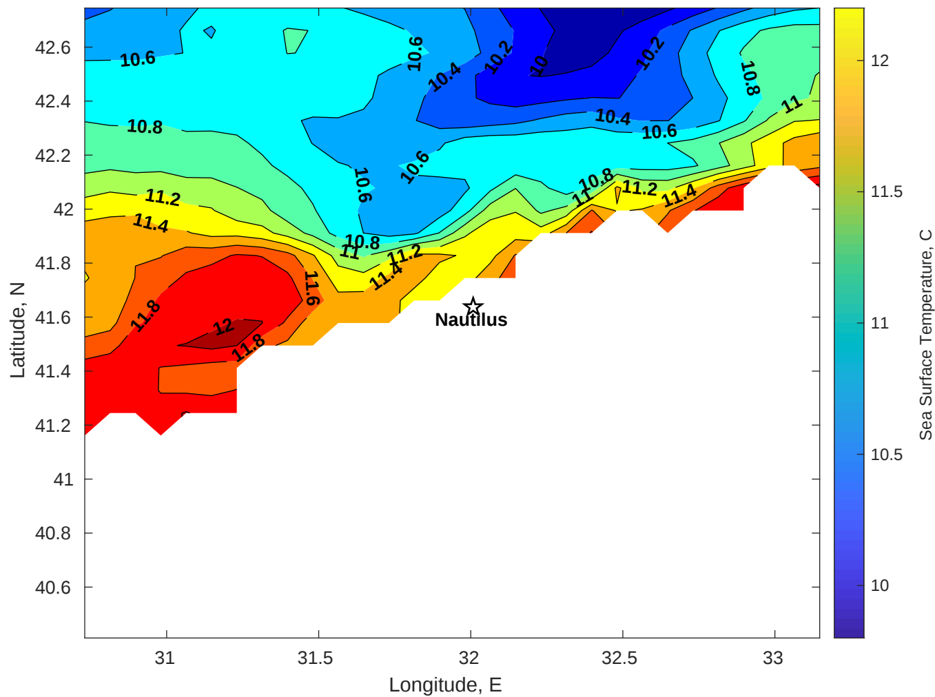
SST for Nautilus at 06-Jan-2026 00:00:00
