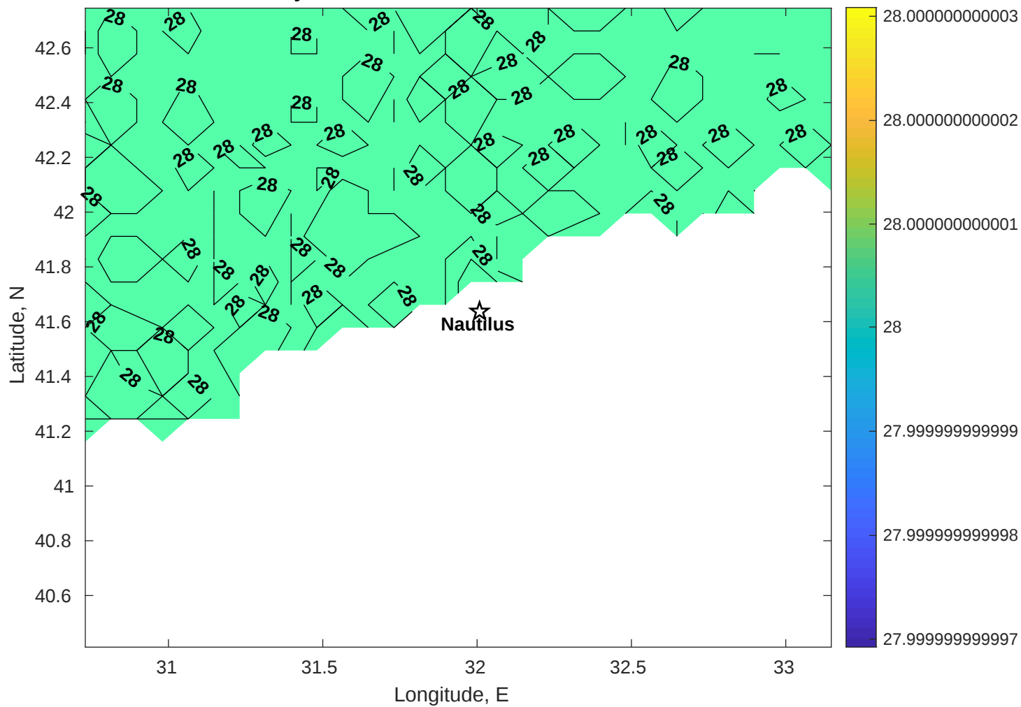
Surface Salinity for Nautilus at 06-Jan-2026 00:00:00
