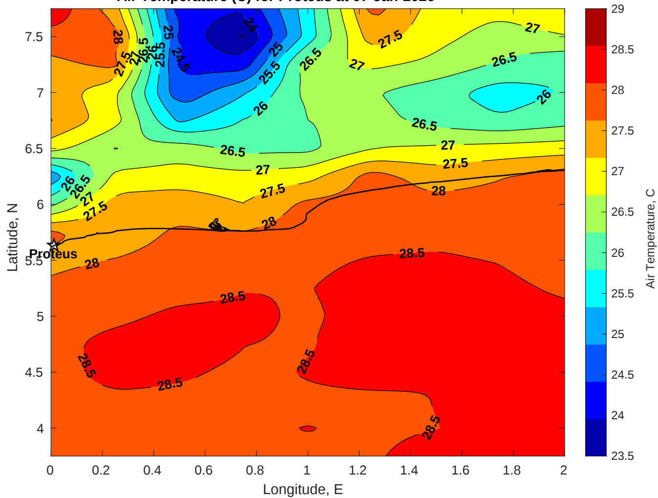
Air Temperature (C) for Proteus at 07-Jan-2026
