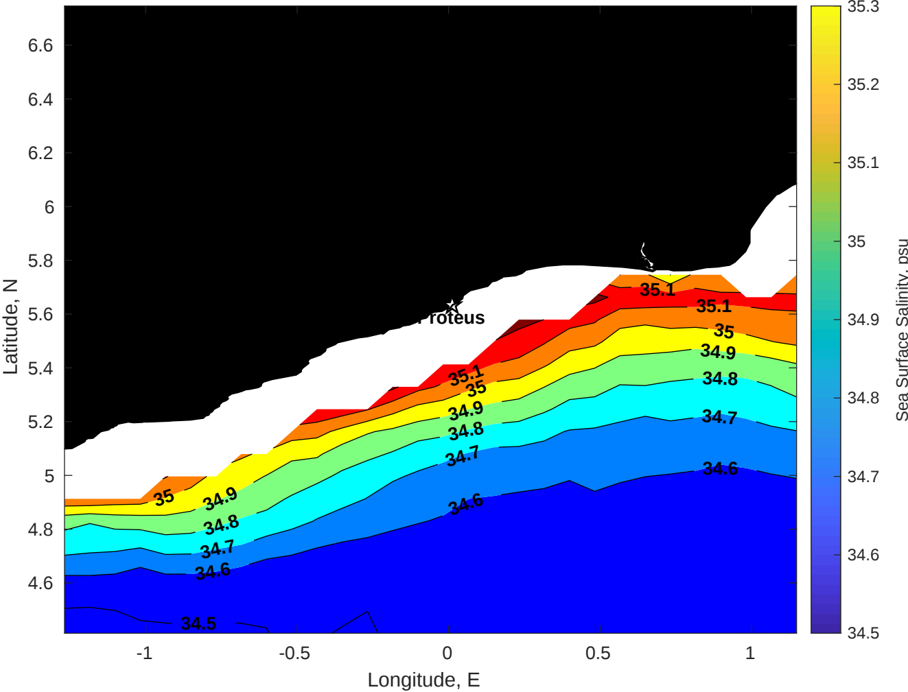
Surface Salinity for Proteus at 06-Jan-2026 00:00:00
