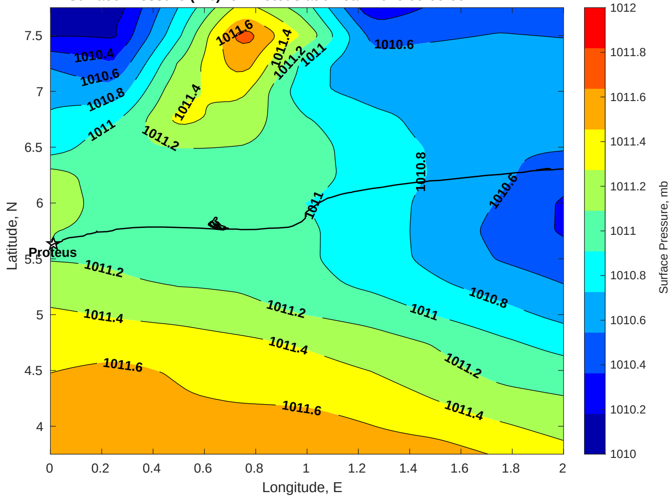
Surface Pressure (mb) for Proteus at 07-Jan-2026 00:00:00
