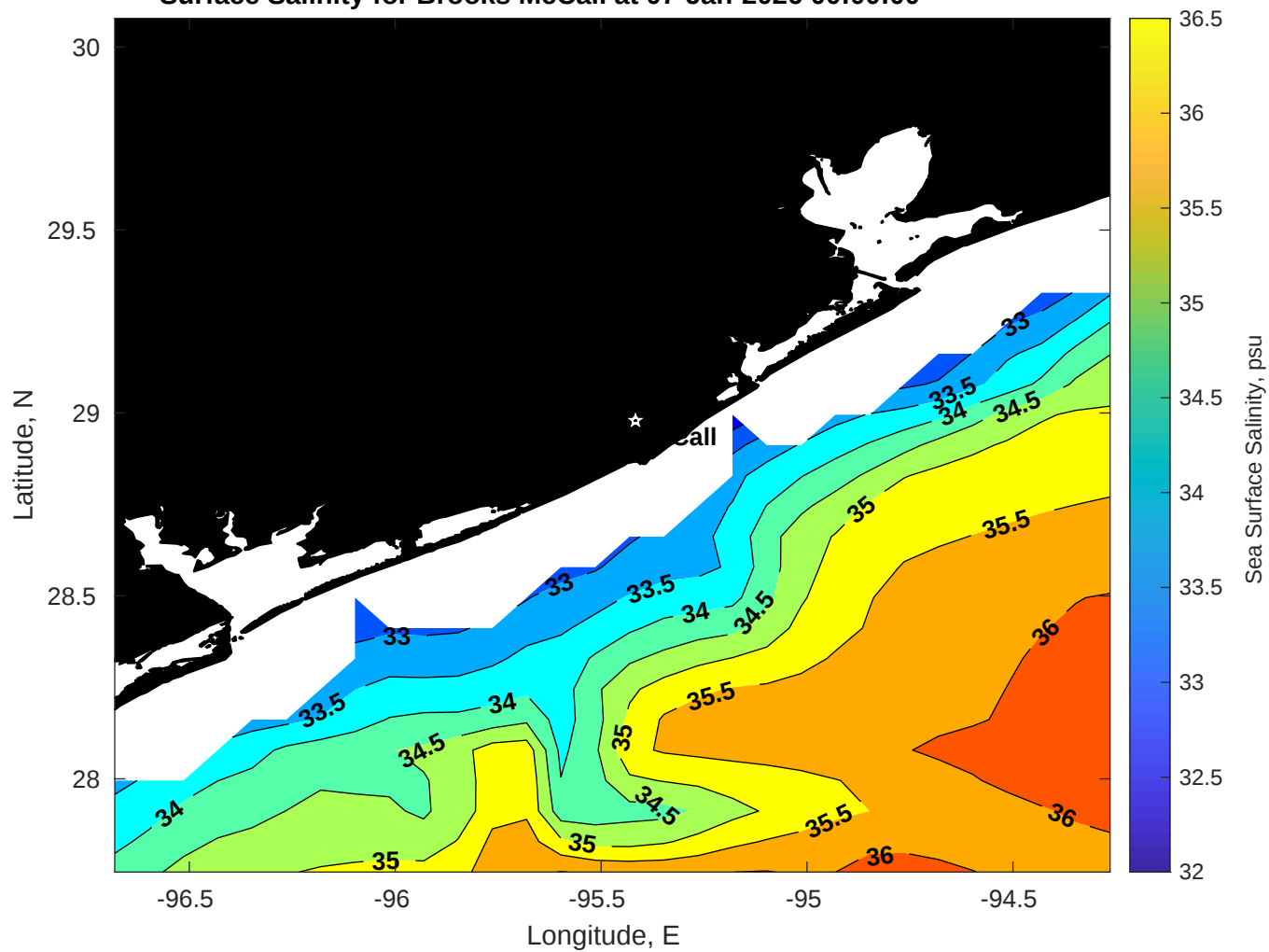
Surface Salinity for Brooks McCall at 07-Jan-2026 00:00:00
