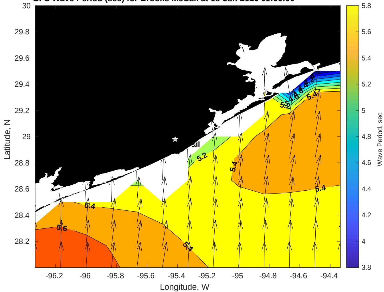
GFS Wave Period (sec) for Brooks McCall at 08-Jan-2026 09:00:00
