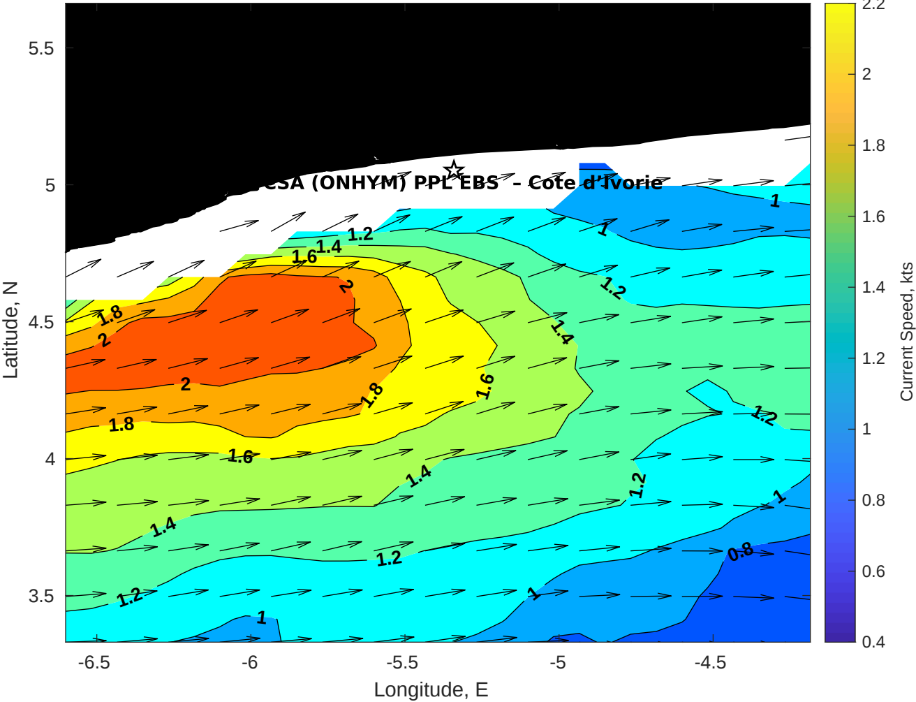
Surface Currents for CSA (ONHYM) PPL EBS - Cote d'Ivoire at 07-Jan-2026 00:00:00
