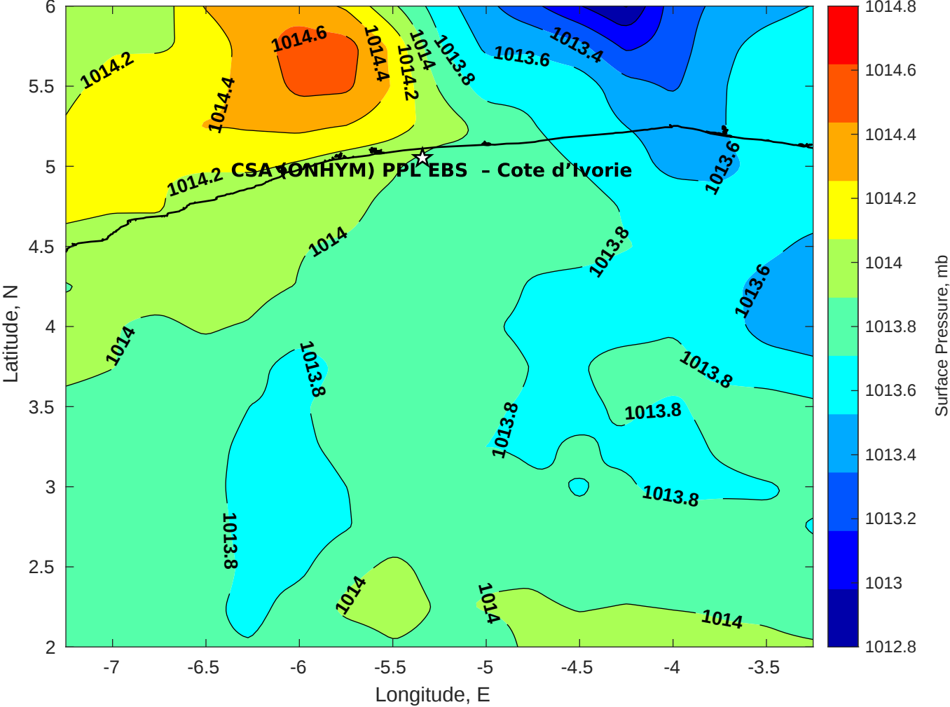
Surface Pressure (mb) for CSA (ONHYM) PPL EBS - Cote d'Ivoire at 09-Jan-2026 00:00:00
