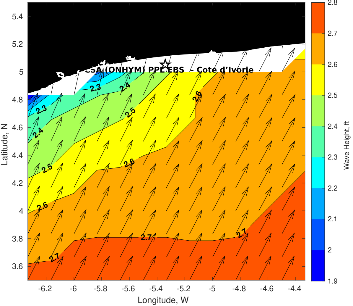
GFS Wave Height (ft) for CSA (ONHYM) PPL EBS - Cote d'Ivoire at 08-Jan-2026 09:00:00
