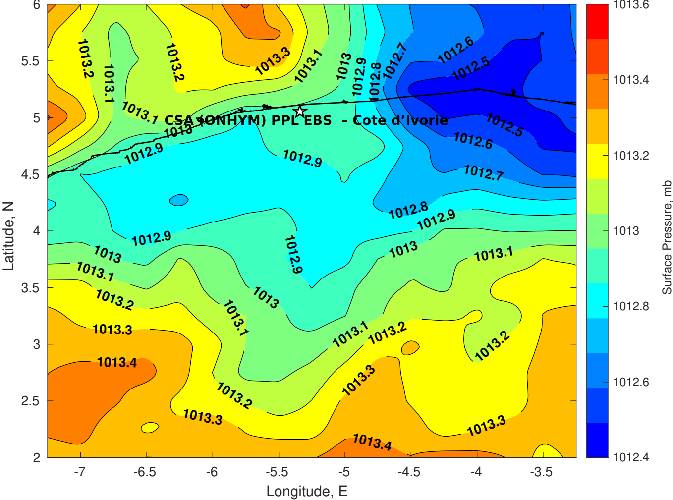
Surface Pressure (mb) for CSA (ONHYM) PPL EBS - Cote d'Ivoire at 08-Jan-2026 00:00:00
