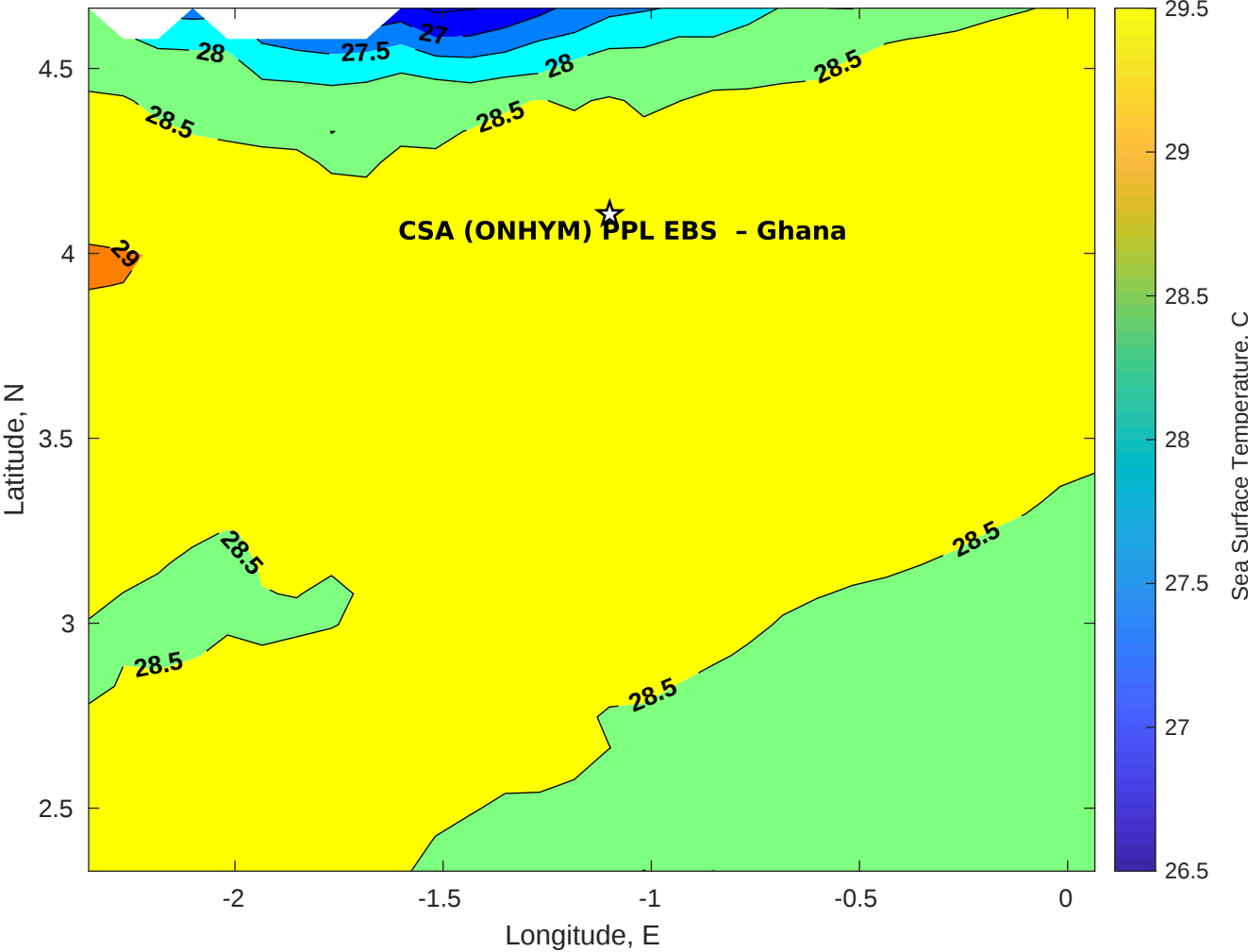
SST for CSA (ONHYM) PPL EBS - Ghana at 07-Jan-2026 00:00:00
