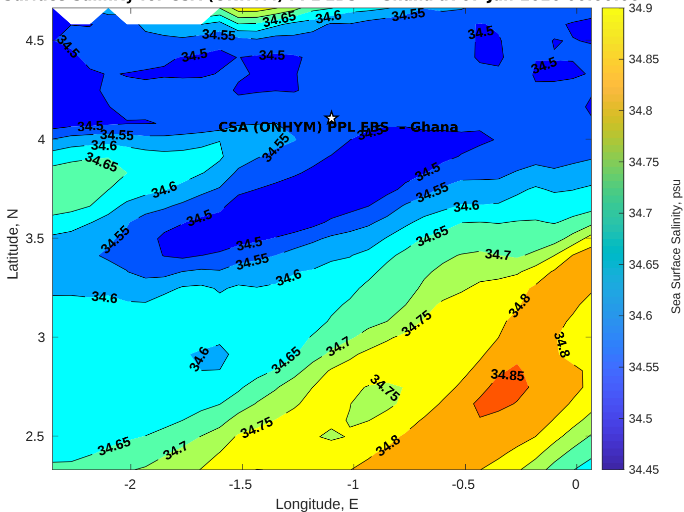
Surface Salinity for CSA (ONHYM) PPL EBS - Ghana at 07-Jan-2026 00:00:00
