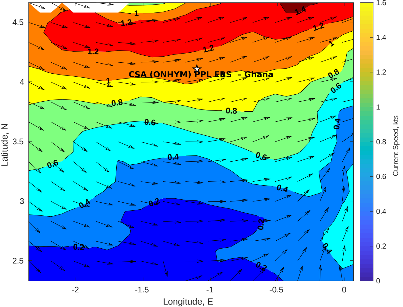
Surface Currents for CSA (ONHYM) PPL EBS - Ghana at 07-Jan-2026 00:00:00
