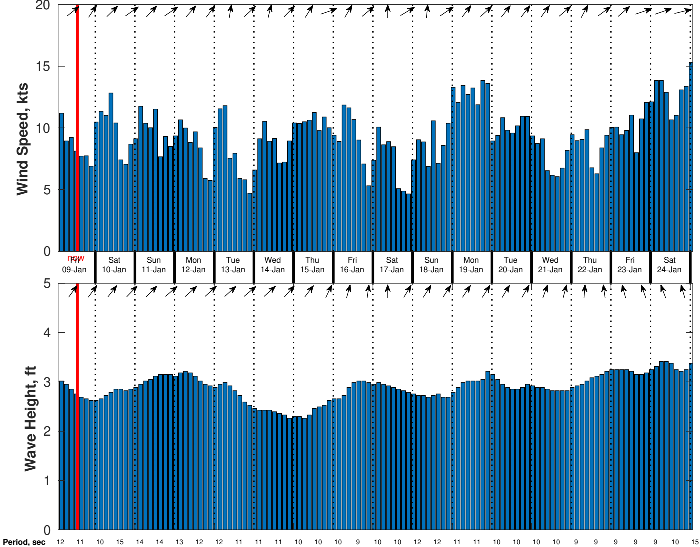
Wind & Wave Forecast for CSA (ONHYM) PPL EBS - Ghana from 08-Jan-2026 02:00:00 to 24-Jan-2026 02:00:00
