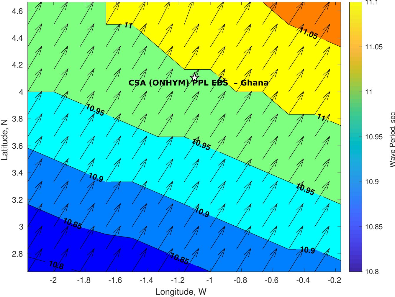
GFS Wave Period (sec) for CSA (ONHYM) PPL EBS - Ghana at 08-Jan-2026 09:00:00
