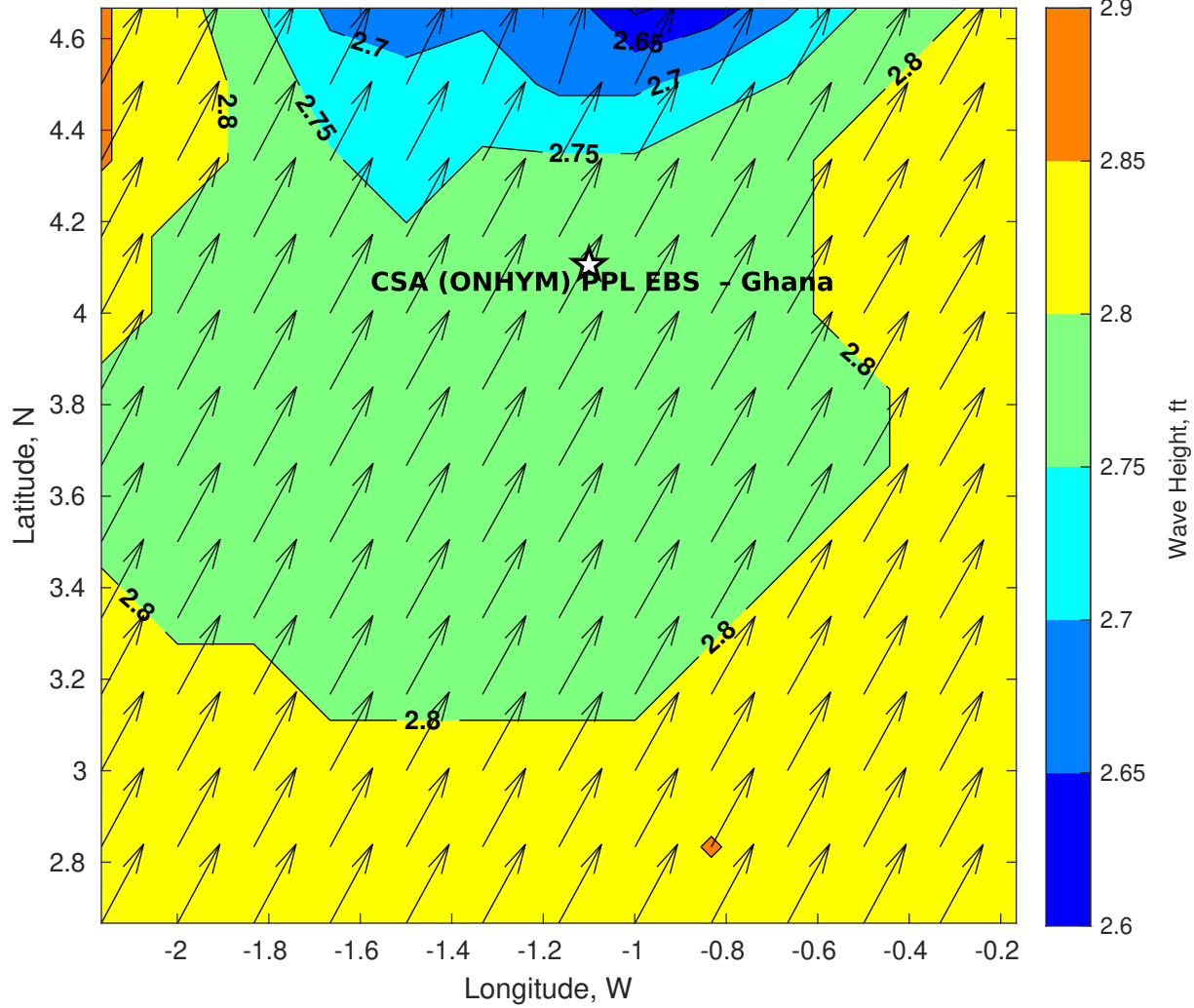
GFS Wave Height (ft) for CSA (ONHYM) PPL EBS - Ghana at 08-Jan-2026 09:00:00
