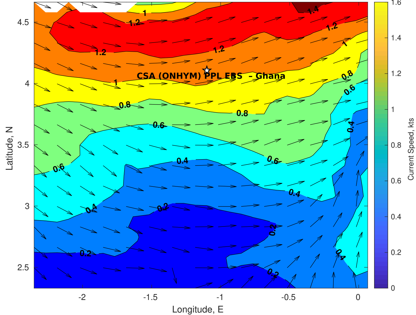
Surface Currents for CSA (ONHYM) PPL EBS - Ghana at 07-Jan-2026 00:00:00
