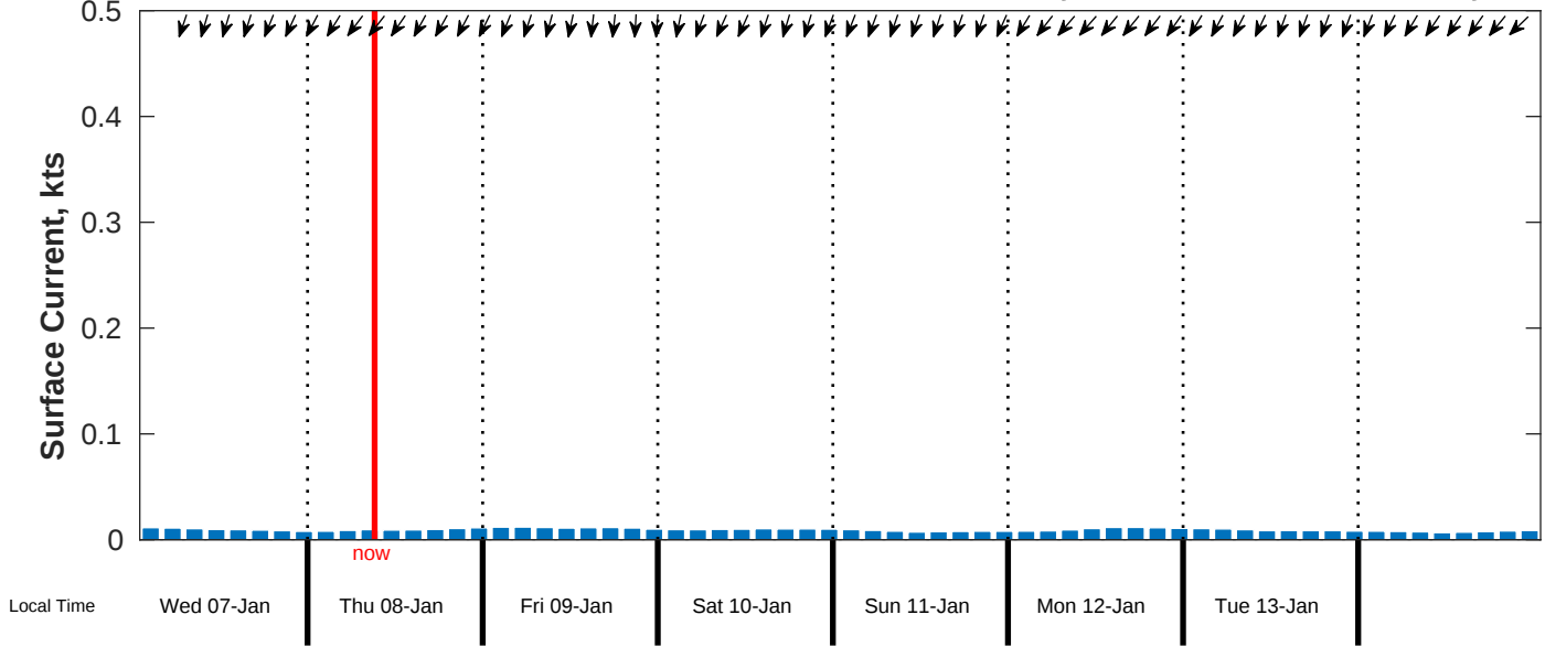
Surface Current Forecast for CSA (ONHYM) PPL EBS - Ghana from 07-Jan-2026 00:00:00 to 15-Jan-2026 00:00:00
