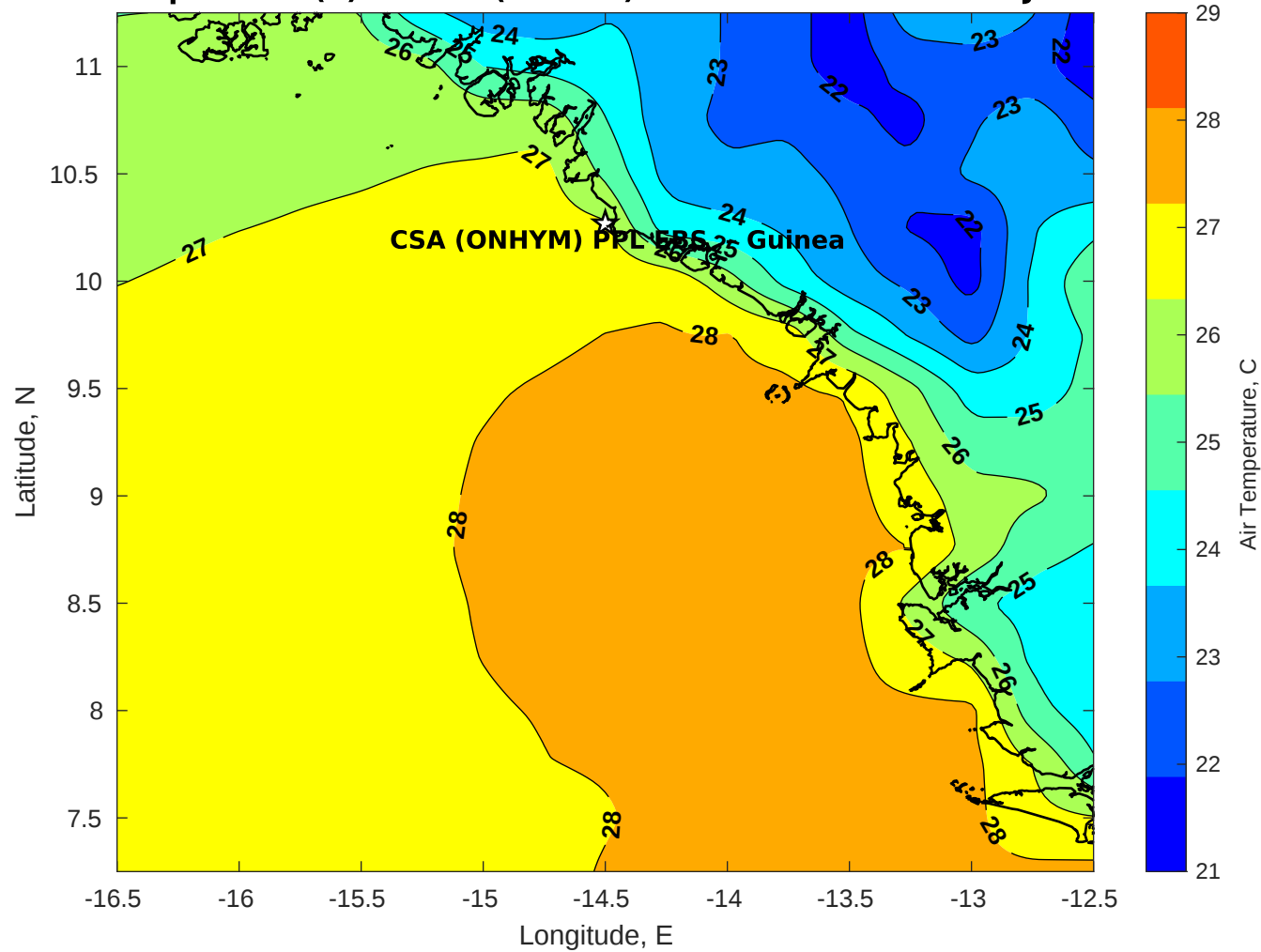
Air Temperature (C) for CSA (ONHYM) PPL EBS - Guinea at 08-Jan-2026
