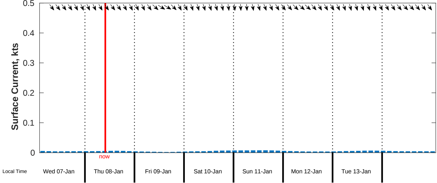
Surface Current Forecast for CSA (ONHYM) PPL EBS - Liberia from 07-Jan-2026 00:00:00 to 15-Jan-2026 00:00:00
