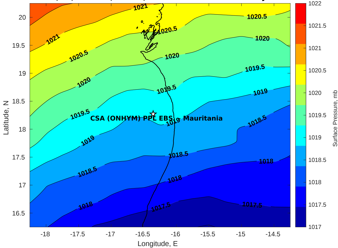
Surface Pressure (mb) for CSA (ONHYM) PPL EBS - Mauritania at 08-Jan-2026 00:00:00
