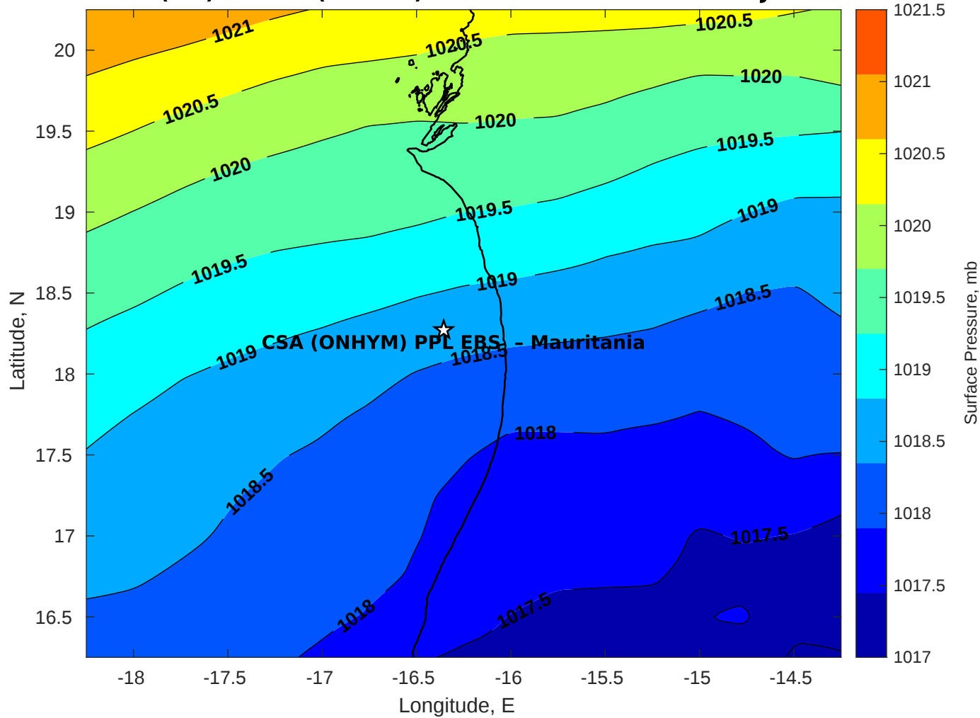
Surface Pressure (mb) for CSA (ONHYM) PPL EBS - Mauritania at 10-Jan-2026 00:00:00
