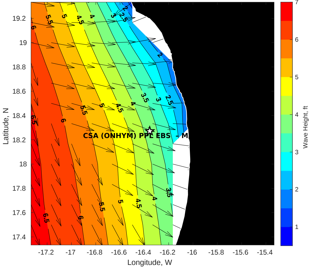
GFS Wave Height (ft) for CSA (ONHYM) PPL EBS - Mauritania at 08-Jan-2026 09:00:00
