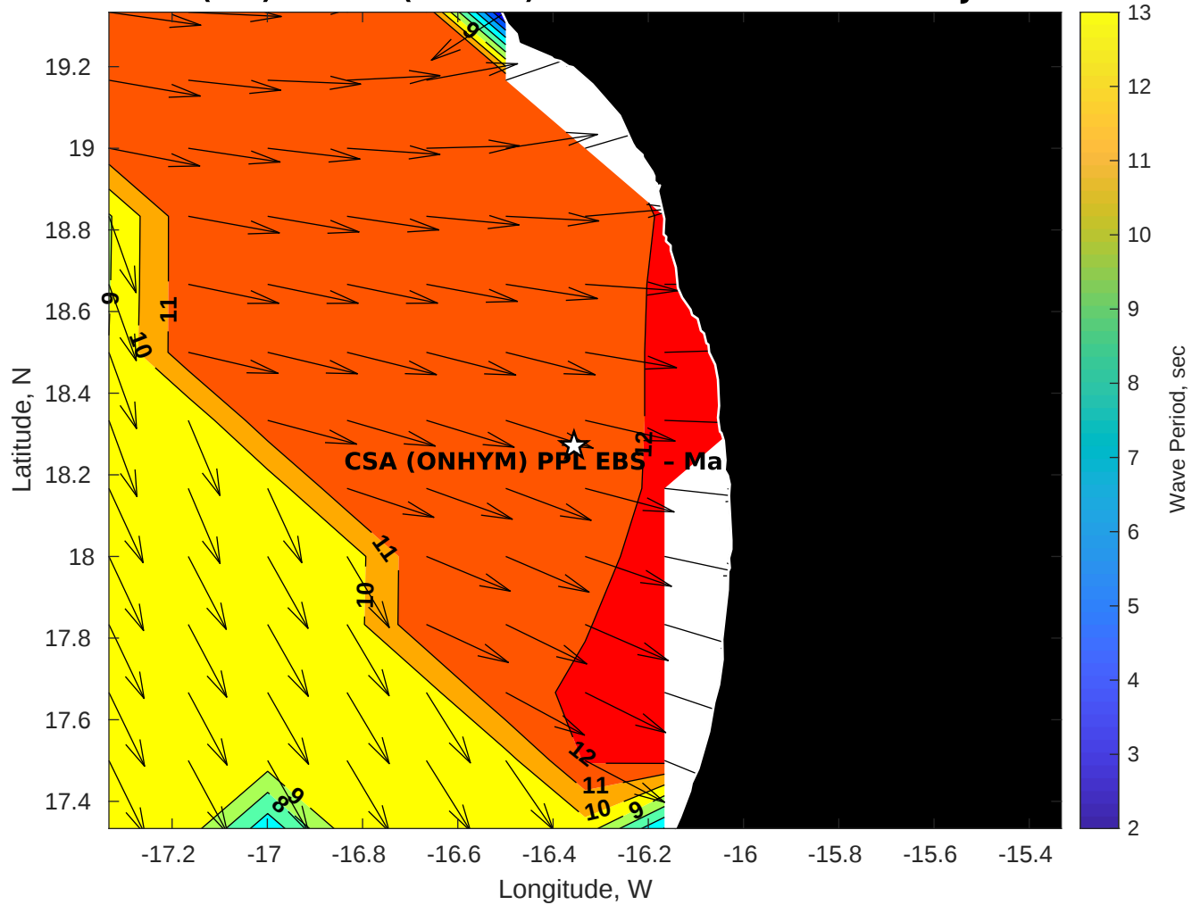
GFS Wave Period (sec) for CSA (ONHYM) PPL EBS - Mauritania at 08-Jan-2026 09:00:00
