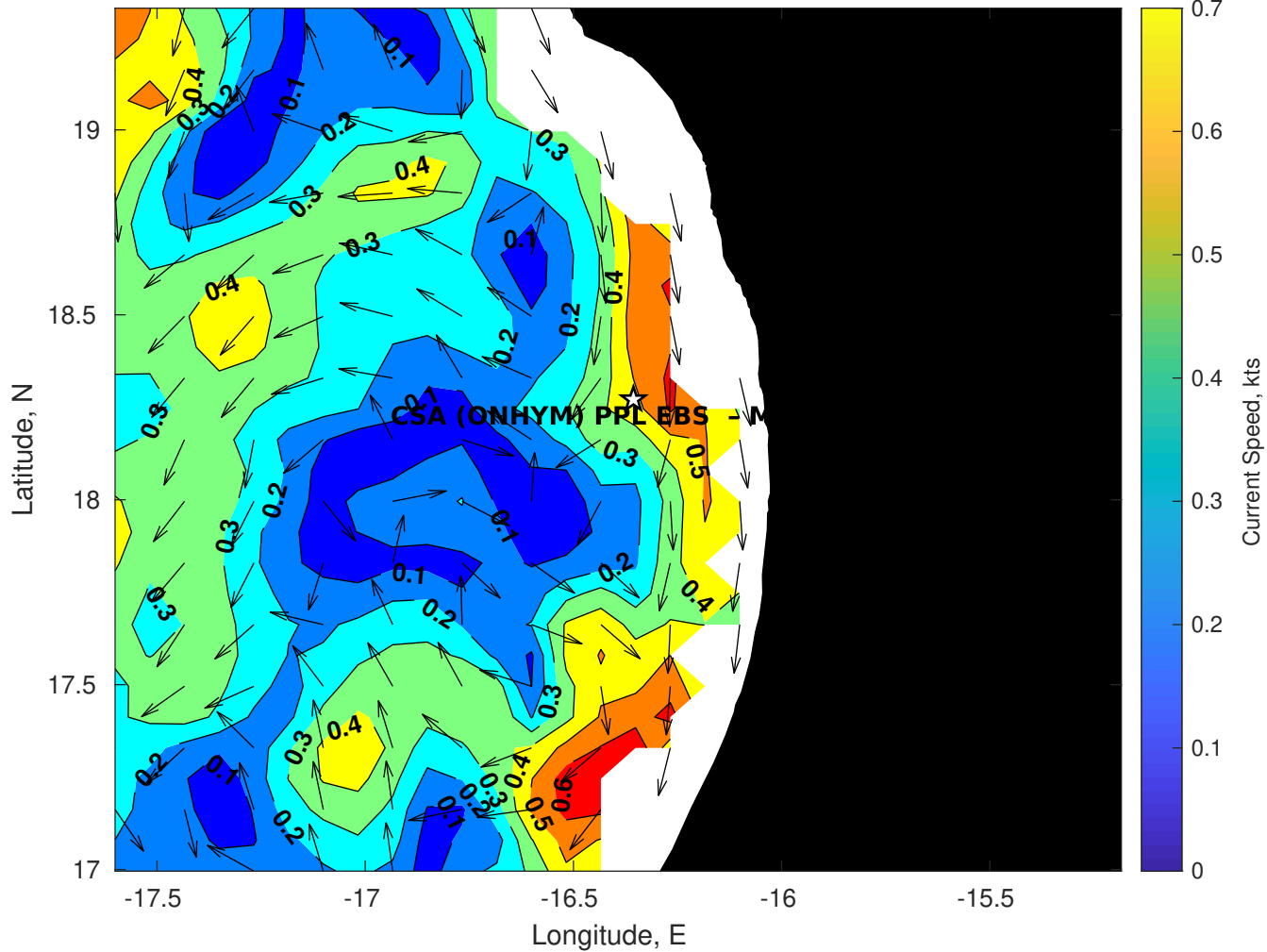
Surface Currents for CSA (ONHYM) PPL EBS - Mauritania at 07-Jan-2026 00:00:00
