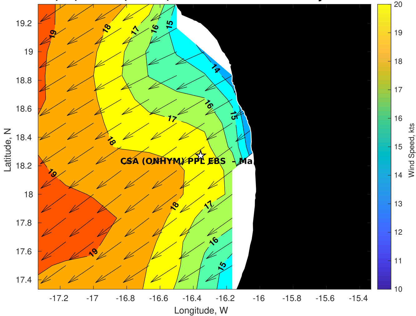
GFS Winds (kts) for CSA (ONHYM) PPL EBS - Mauritania at 08-Jan-2026 09:00:00
