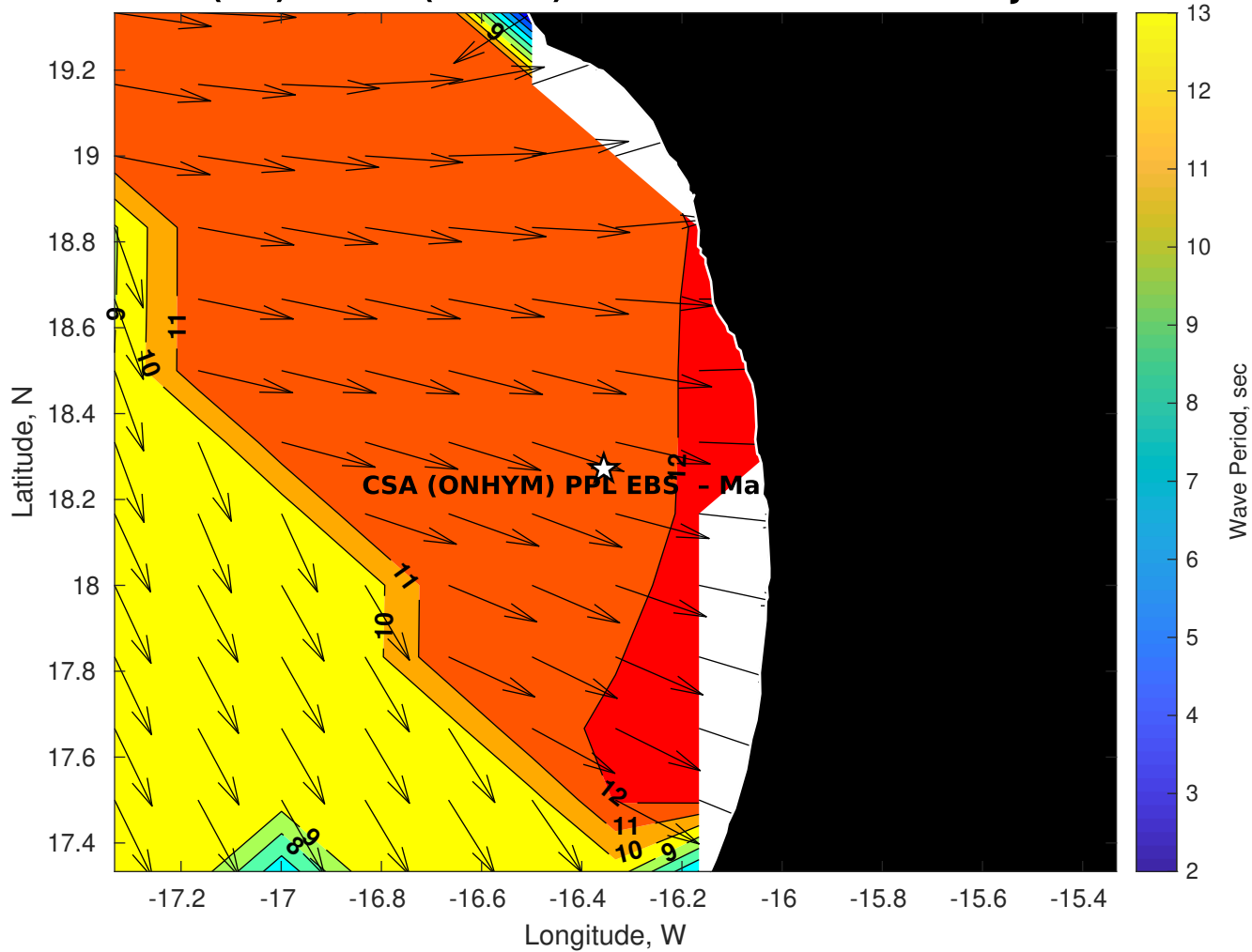
GFS Wave Period (sec) for CSA (ONHYM) PPL EBS - Mauritania at 08-Jan-2026 09:00:00
