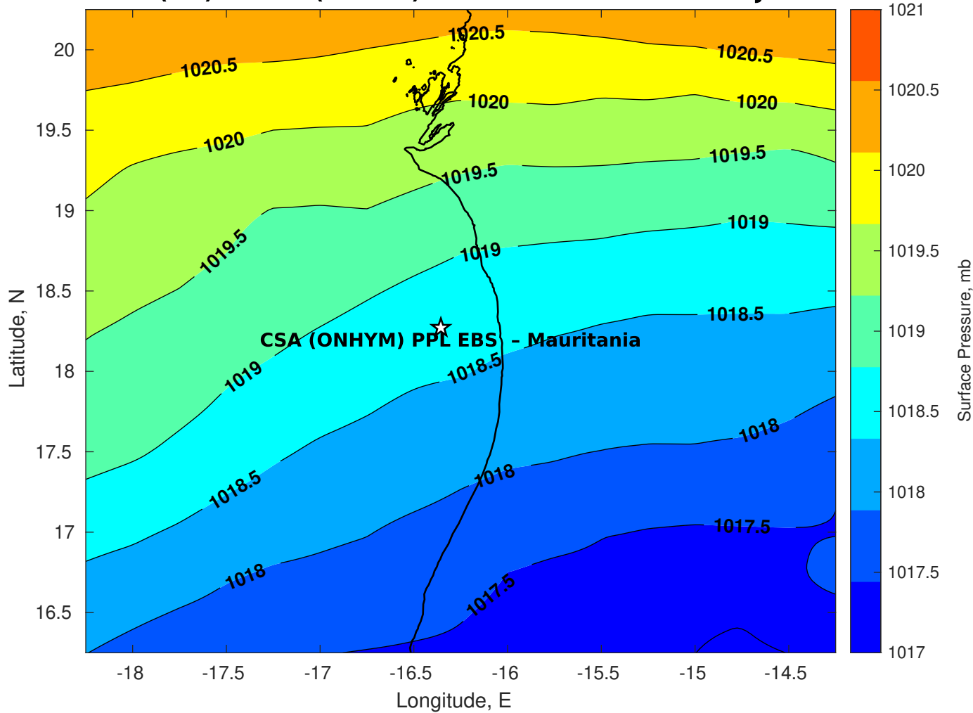
Surface Pressure (mb) for CSA (ONHYM) PPL EBS - Mauritania at 09-Jan-2026 00:00:00
