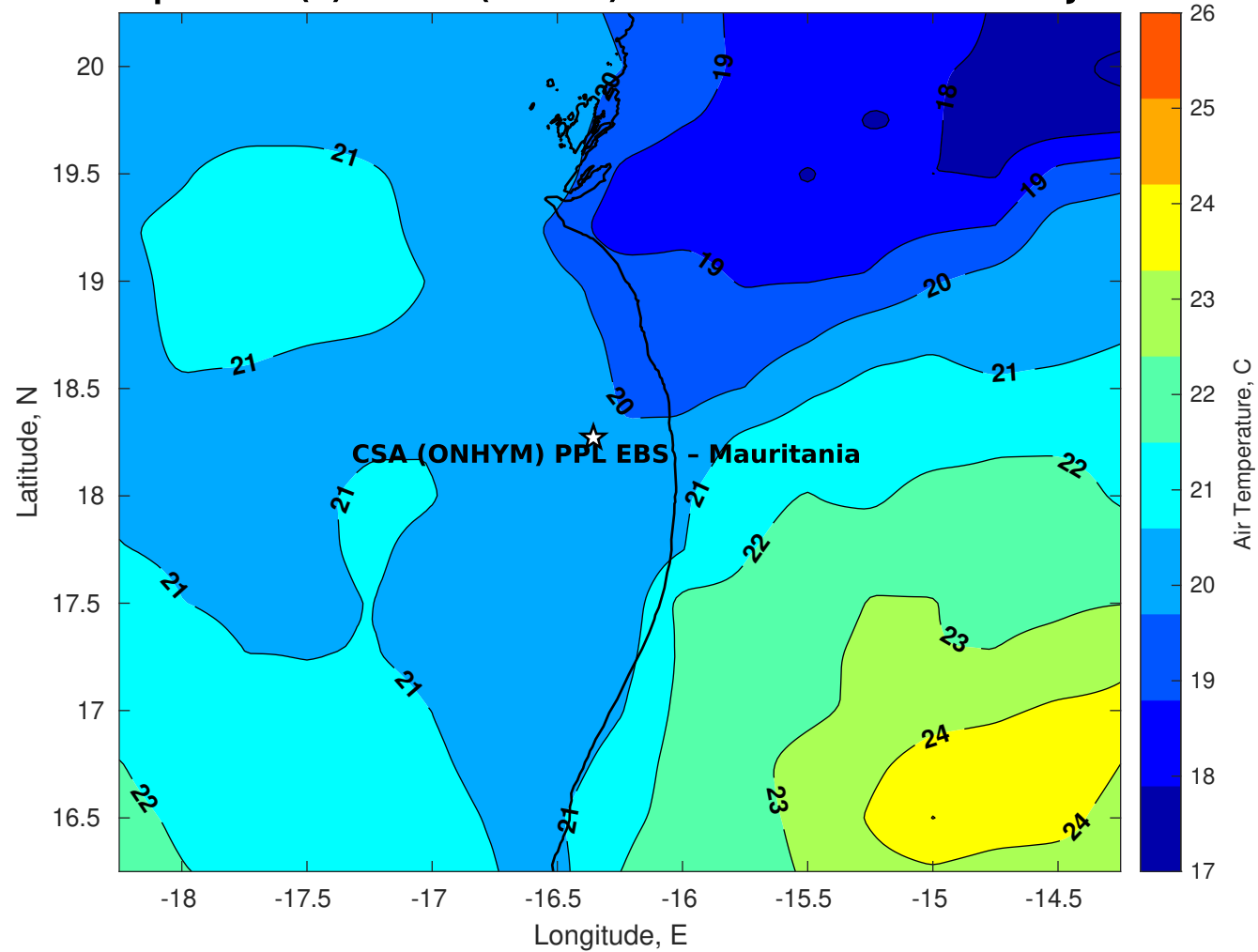
Air Temperature (C) for CSA (ONHYM) PPL EBS - Mauritania at 08-Jan-2026
