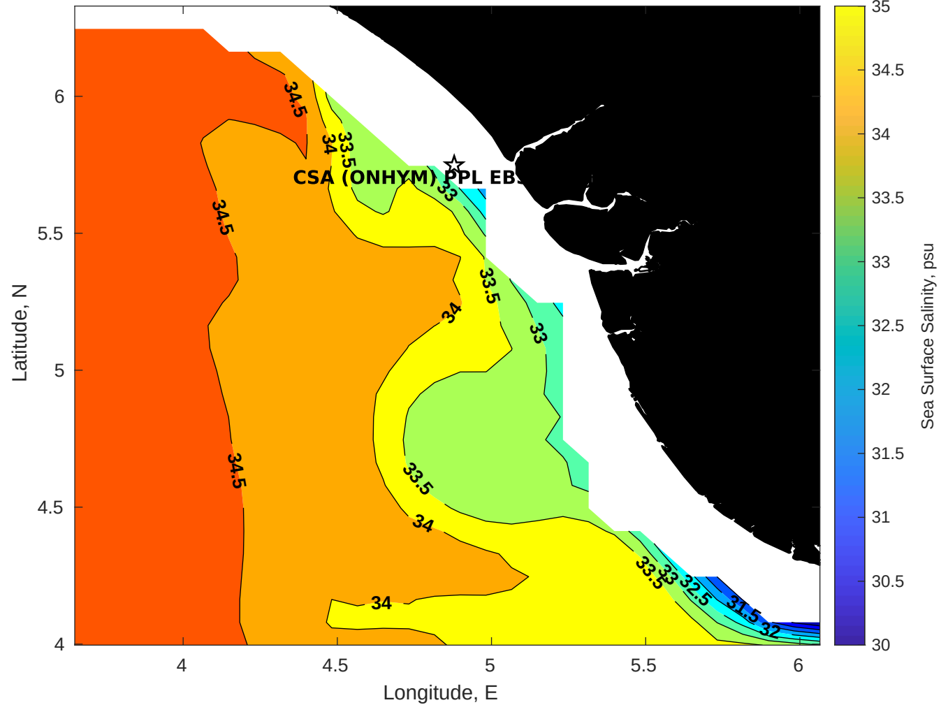
Surface Salinity for CSA (ONHYM) PPL EBS - Nigeria at 07-Jan-2026 00:00:00
