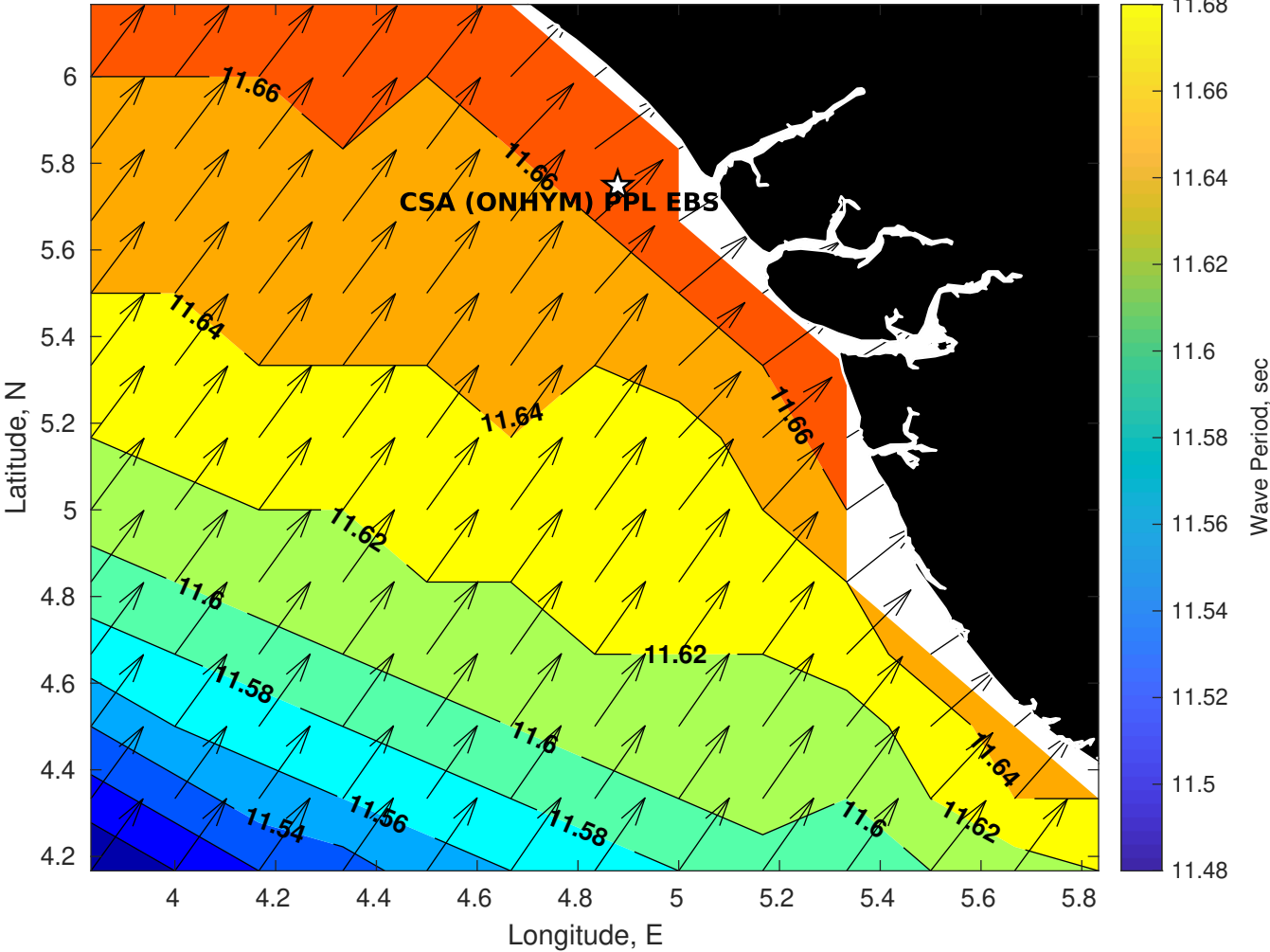
GFS Wave Period (sec) for CSA (ONHYM) PPL EBS - Nigeria at 08-Jan-2026 09:00:00
