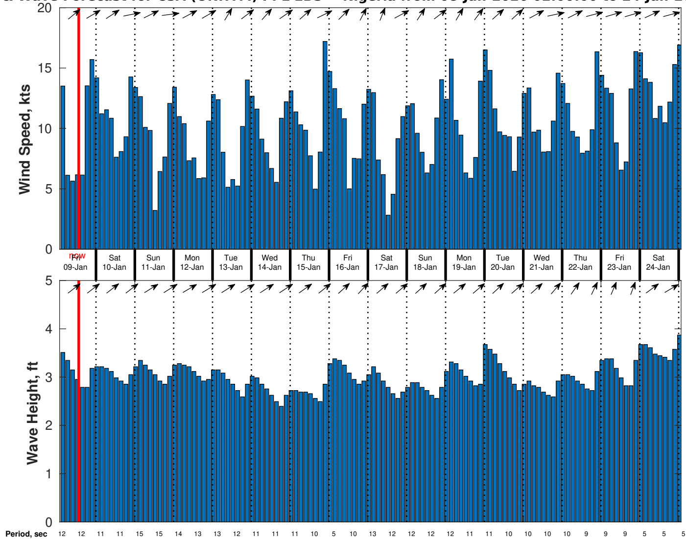
Wind & Wave Forecast for CSA (ONHYM) PPL EBS - Nigeria from 08-Jan-2026 02:00:00 to 24-Jan-2026 02:00:00
