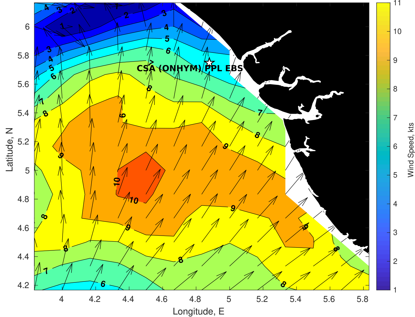
GFS Winds (kts) for CSA (ONHYM) PPL EBS - Nigeria at 08-Jan-2026 09:00:00
