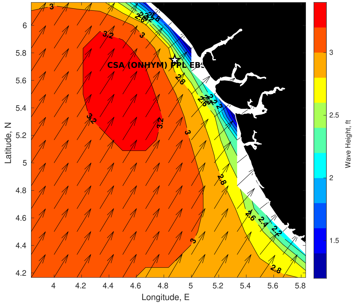
GFS Wave Height (ft) for CSA (ONHYM) PPL EBS - Nigeria at 08-Jan-2026 09:00:00
