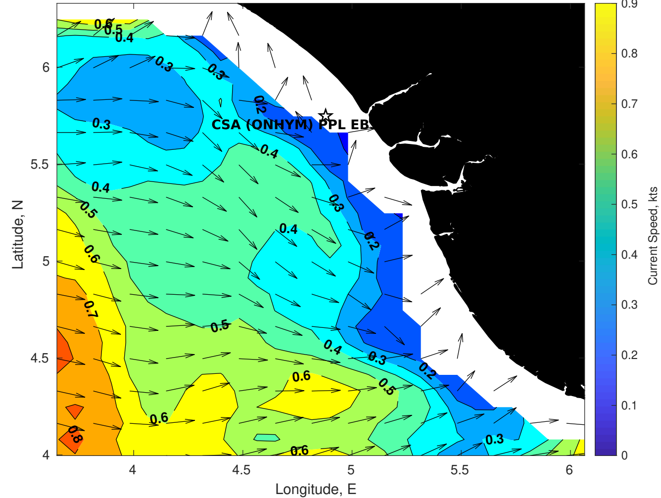
Surface Currents for CSA (ONHYM) PPL EBS - Nigeria at 07-Jan-2026 00:00:00
