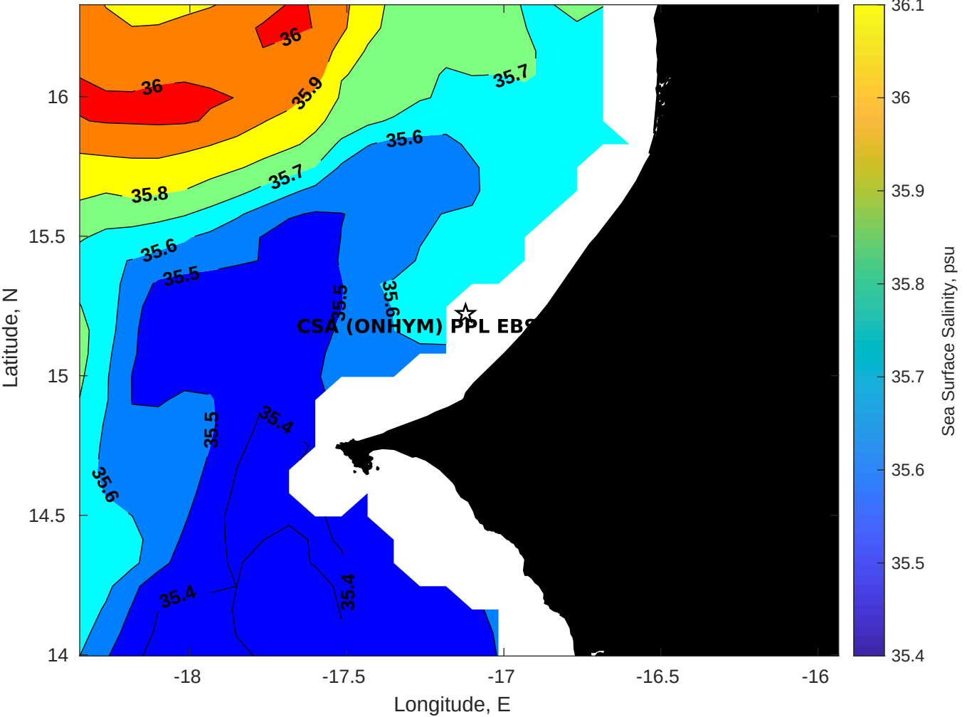
Surface Salinity for CSA (ONHYM) PPL EBS - Senegal at 07-Jan-2026 00:00:00
