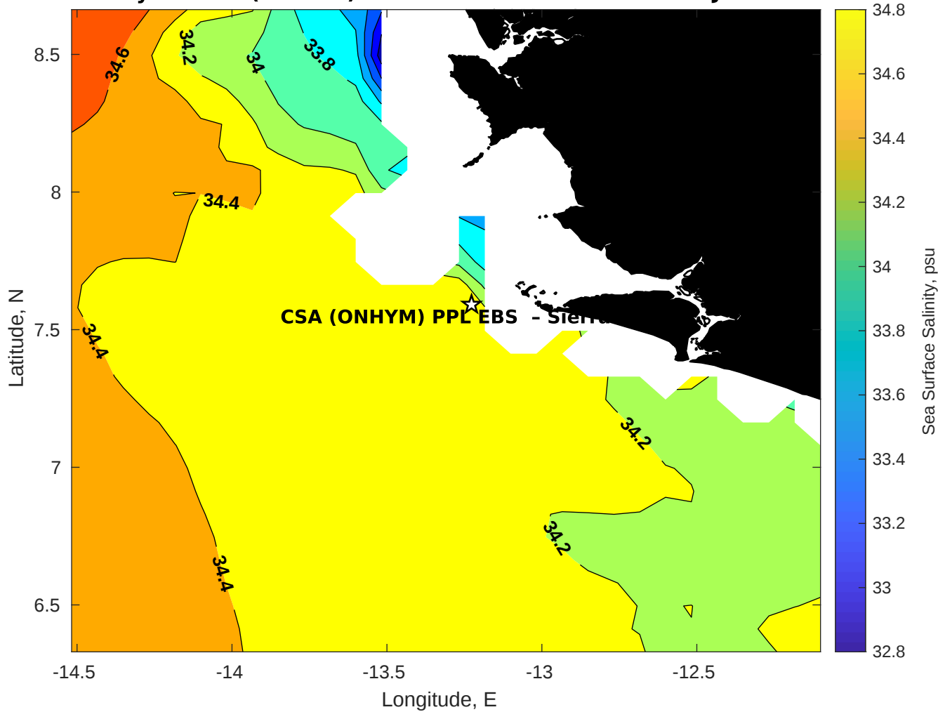
Surface Salinity for CSA (ONHYM) PPL EBS - Sierra Leone at 07-Jan-2026 00:00:00
