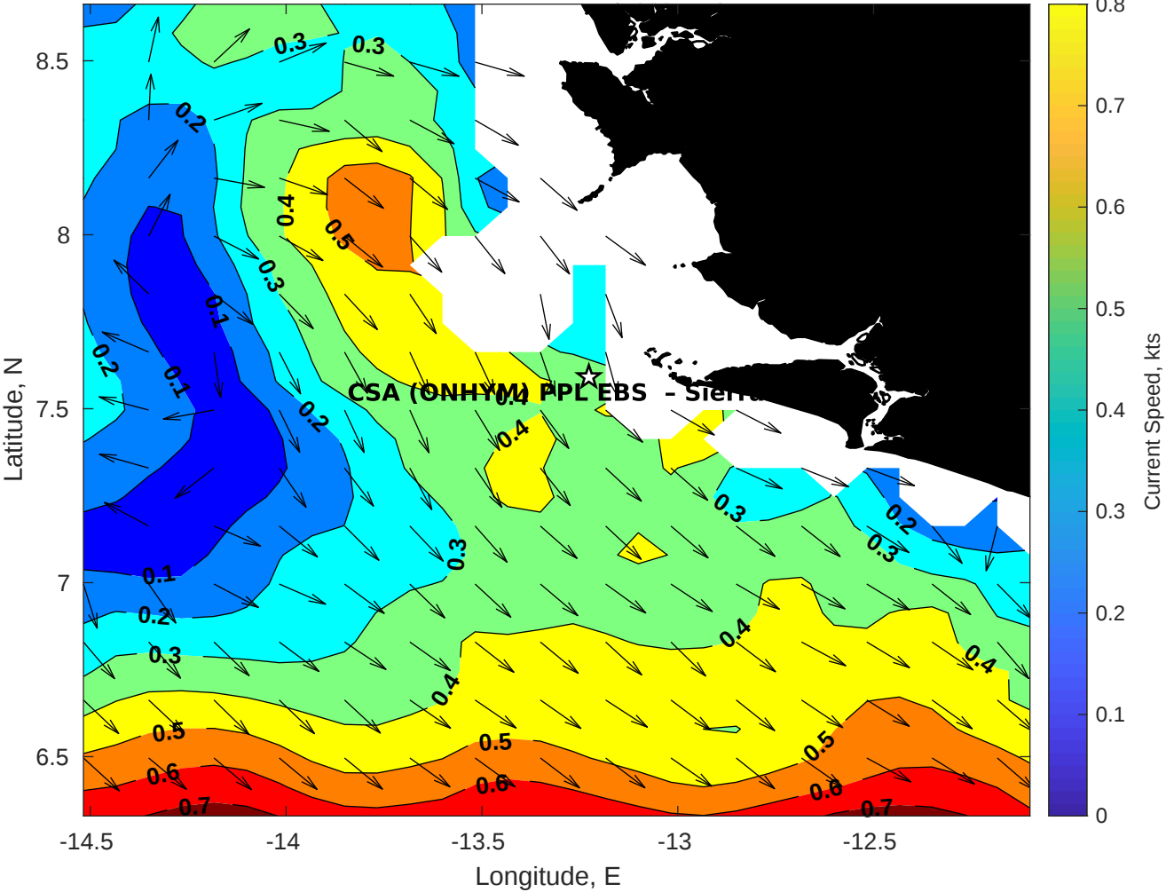
Surface Currents for CSA (ONHYM) PPL EBS - Sierra Leone at 07-Jan-2026 00:00:00
