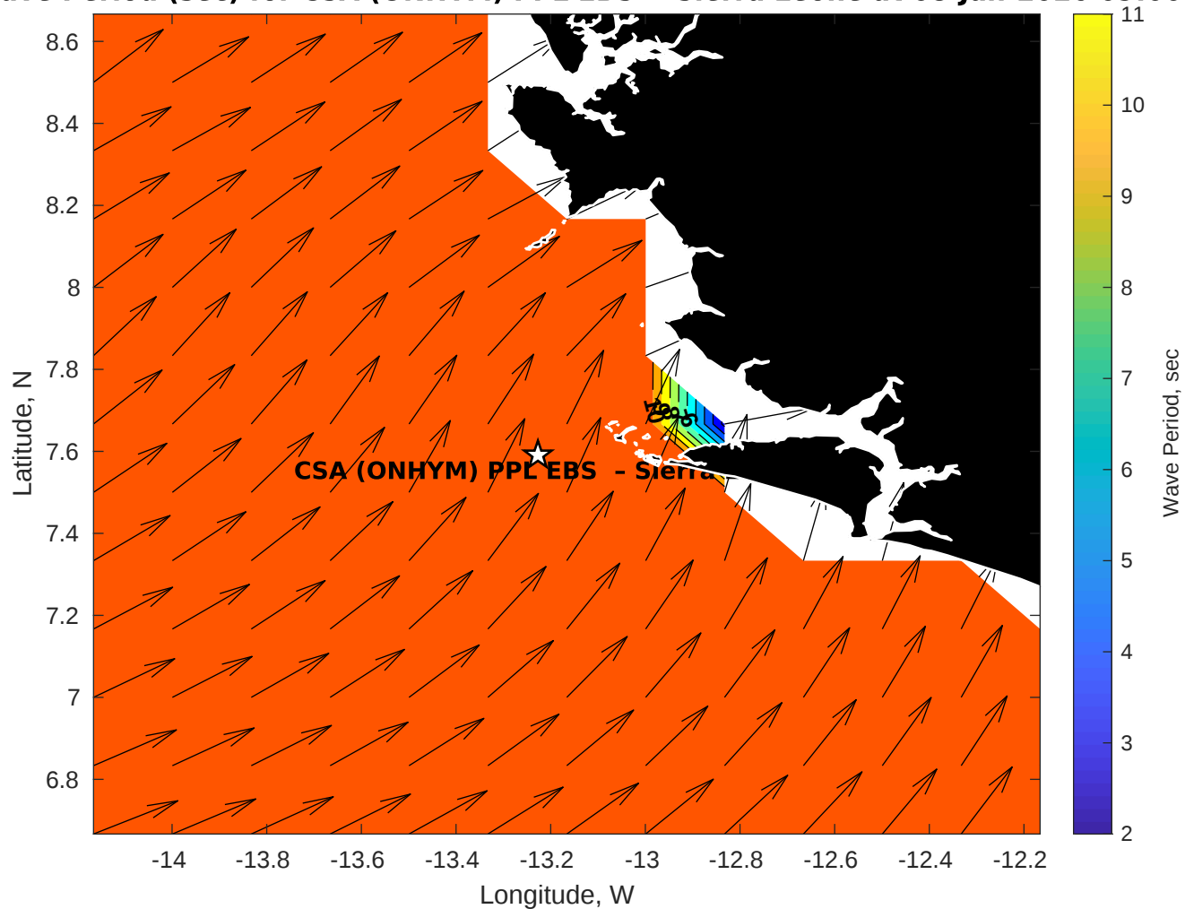
GFS Wave Period (sec) for CSA (ONHYM) PPL EBS - Sierra Leone at 08-Jan-2026 09:00:00
