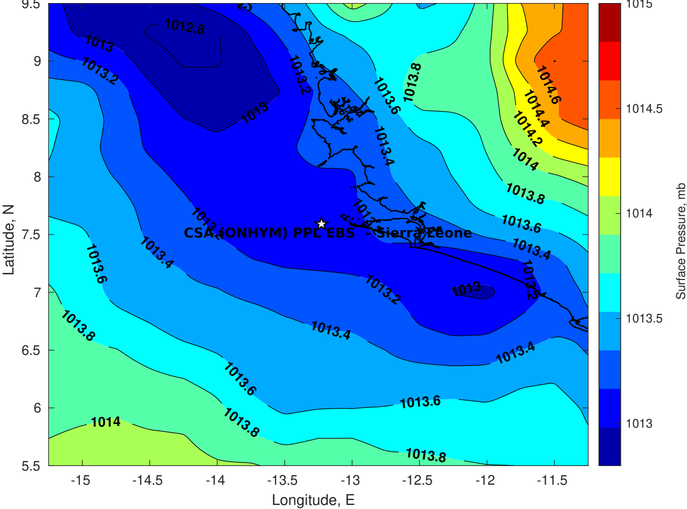
Surface Pressure (mb) for CSA (ONHYM) PPL EBS - Sierra Leone at 09-Jan-2026 00:00:00
