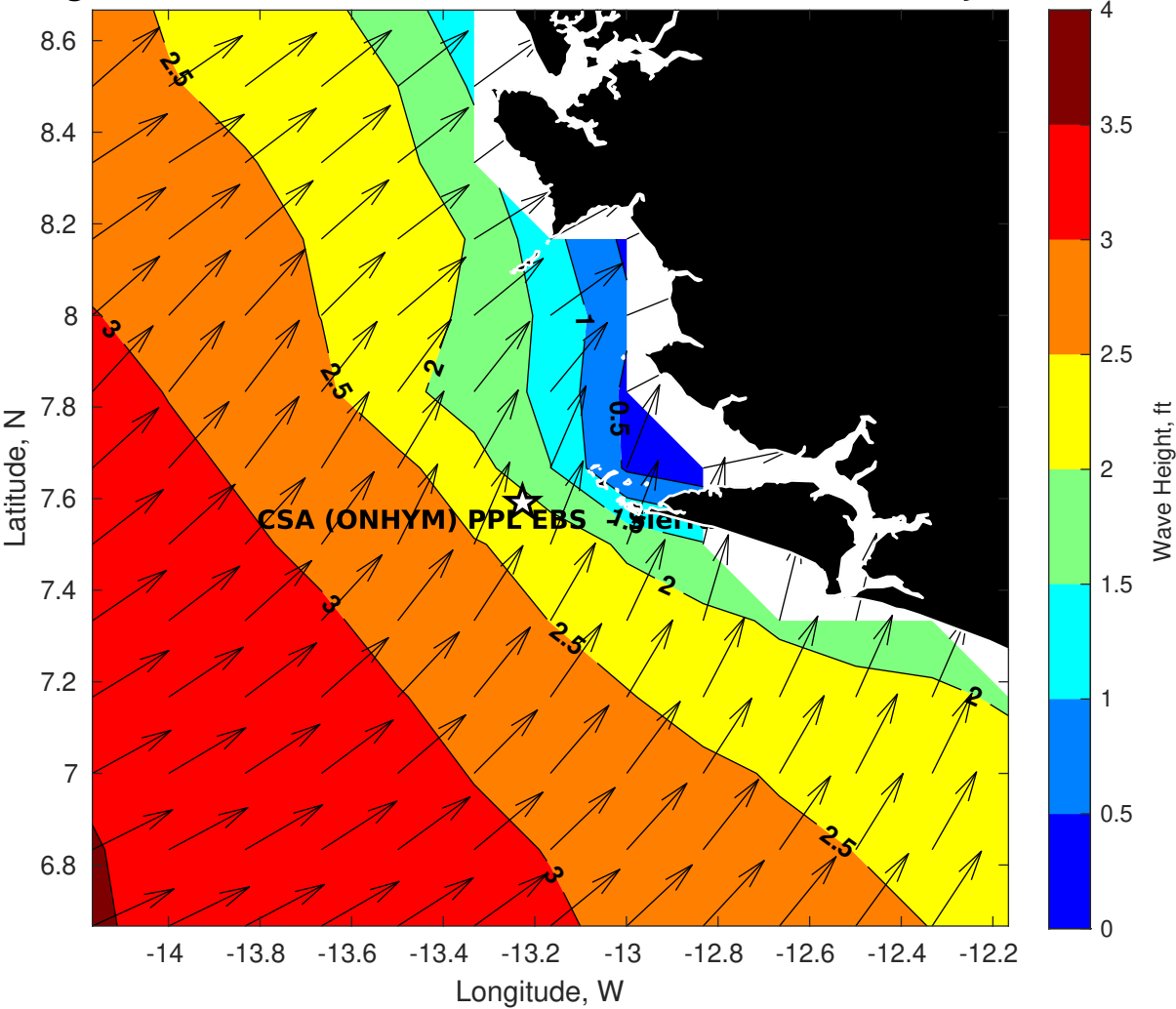
GFS Wave Height (ft) for CSA (ONHYM) PPL EBS - Sierra Leone at 08-Jan-2026 09:00:00
