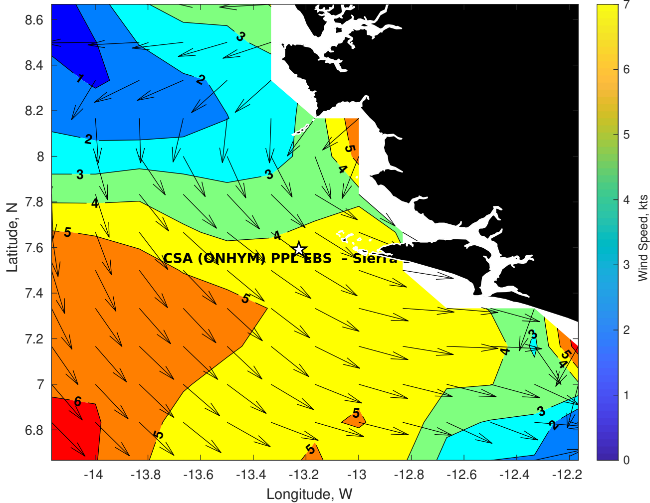
GFS Winds (kts) for CSA (ONHYM) PPL EBS - Sierra Leone at 08-Jan-2026 09:00:00
