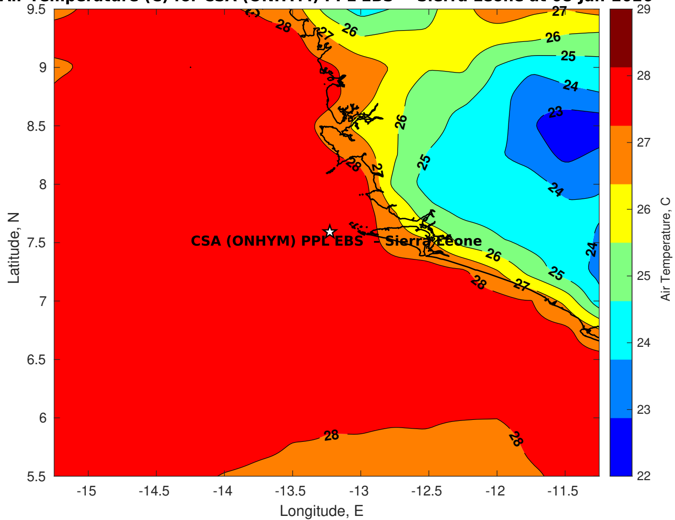
Air Temperature (C) for CSA (ONHYM) PPL EBS - Sierra Leone at 08-Jan-2026
