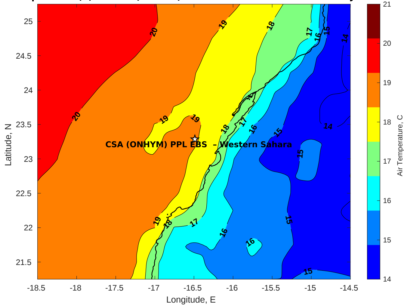
Air Temperature (C) for CSA (ONHYM) PPL EBS - Western Sahara at 08-Jan-2026
