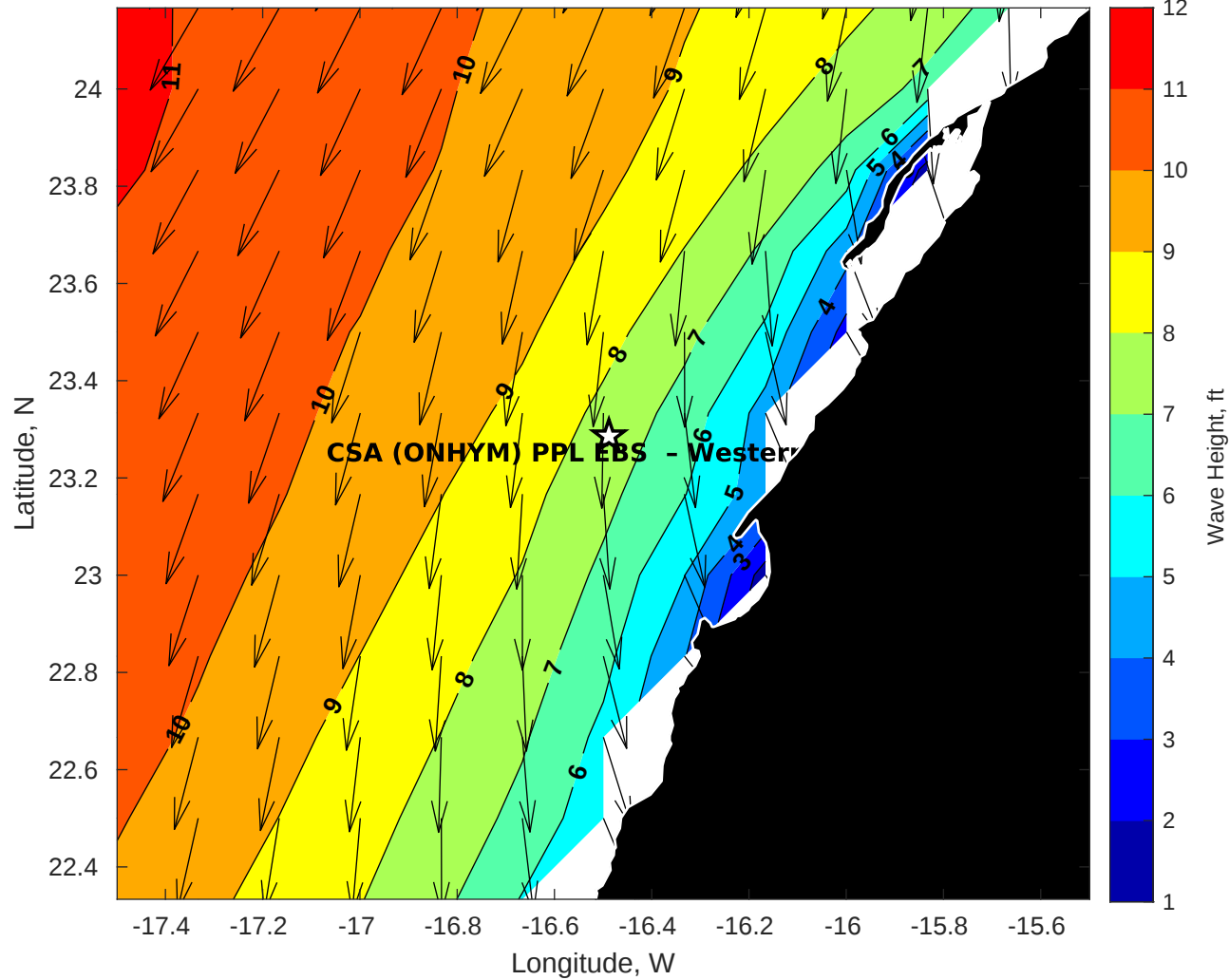
GFS Wave Height (ft) for CSA (ONHYM) PPL EBS - Western Sahara at 08-Jan-2026 09:00:00
