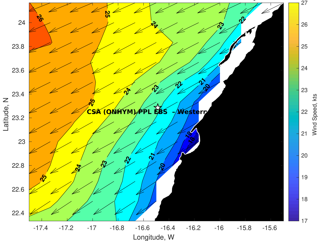
GFS Winds (kts) for CSA (ONHYM) PPL EBS - Western Sahara at 08-Jan-2026 09:00:00
