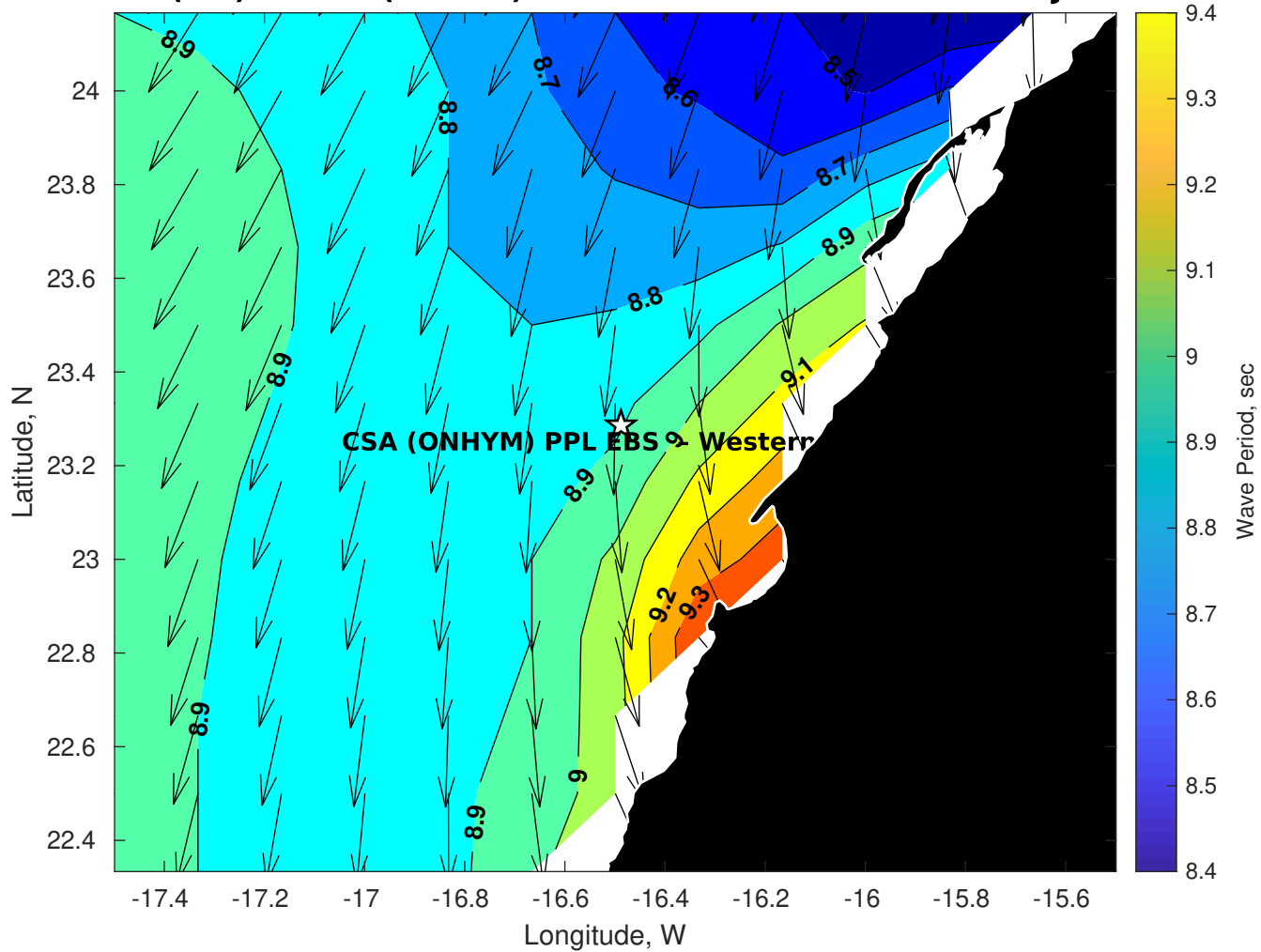
GFS Wave Period (sec) for CSA (ONHYM) PPL EBS - Western Sahara at 08-Jan-2026 09:00:00
