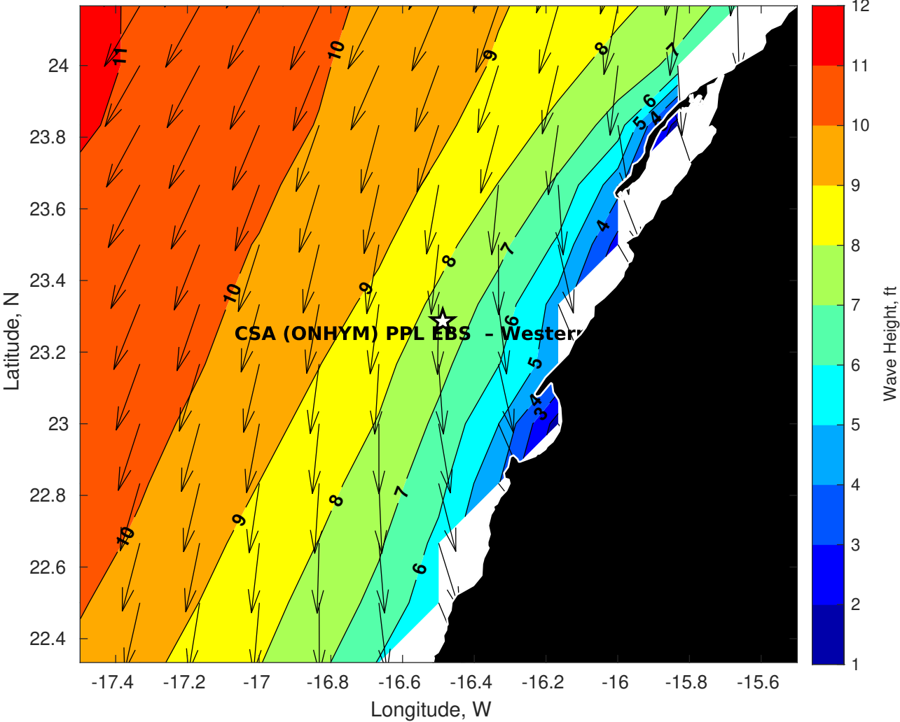
GFS Wave Height (ft) for CSA (ONHYM) PPL EBS - Western Sahara at 08-Jan-2026 09:00:00
