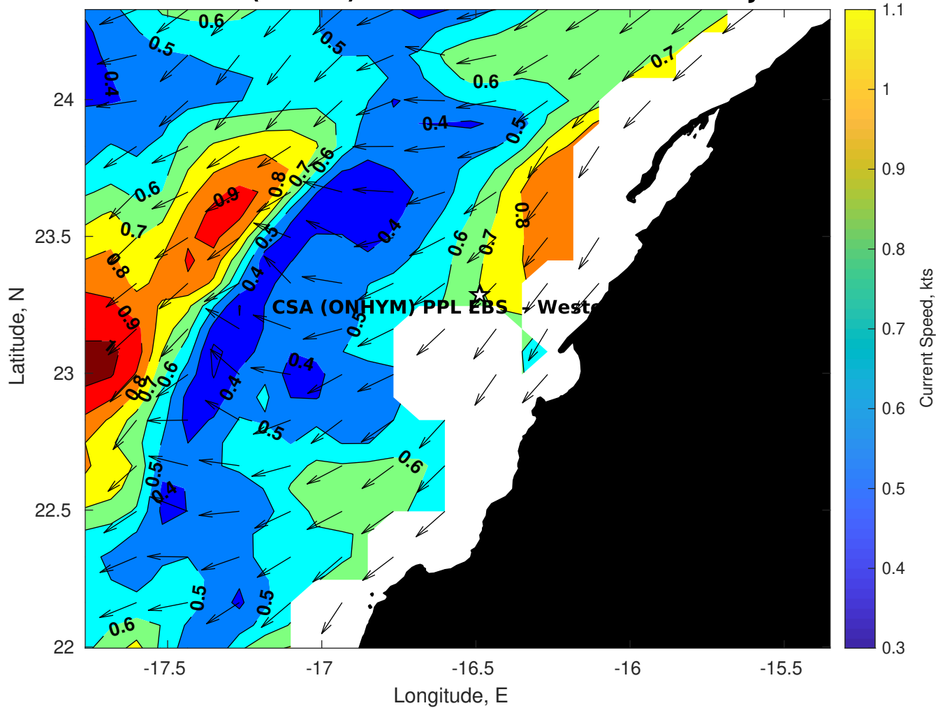
Surface Currents for CSA (ONHYM) PPL EBS - Western Sahara at 07-Jan-2026 00:00:00
