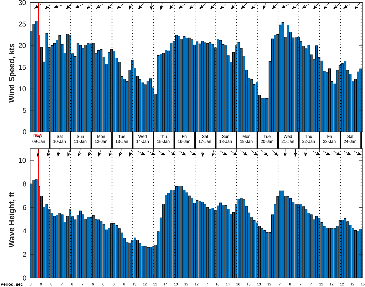
Wind & Wave Forecast for CSA (ONHYM) PPL EBS - Western Sahara from 08-Jan-2026 01:00:00 to 24-Jan-2026 01:00:00
