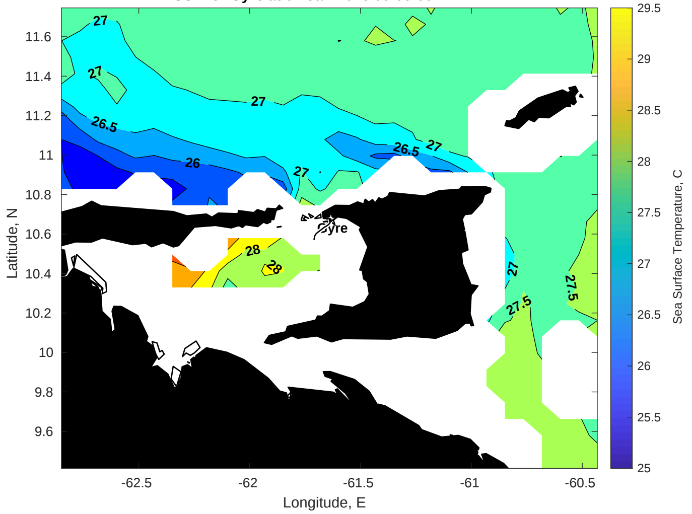
SST for Gyre at 07-Jan-2026 00:00:00
