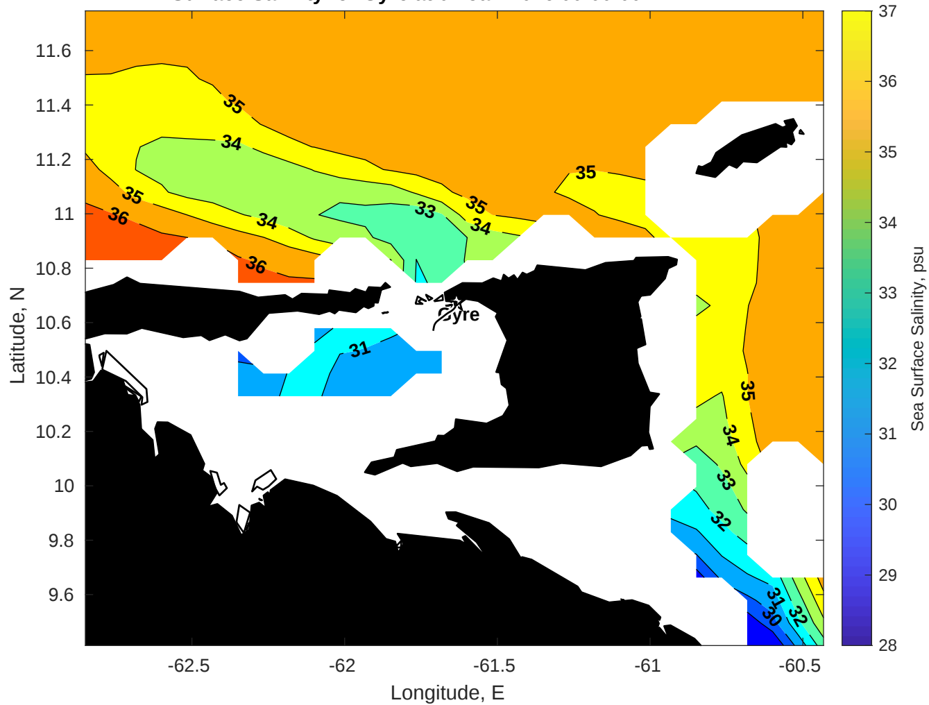
Surface Salinity for Gyre at 07-Jan-2026 00:00:00
